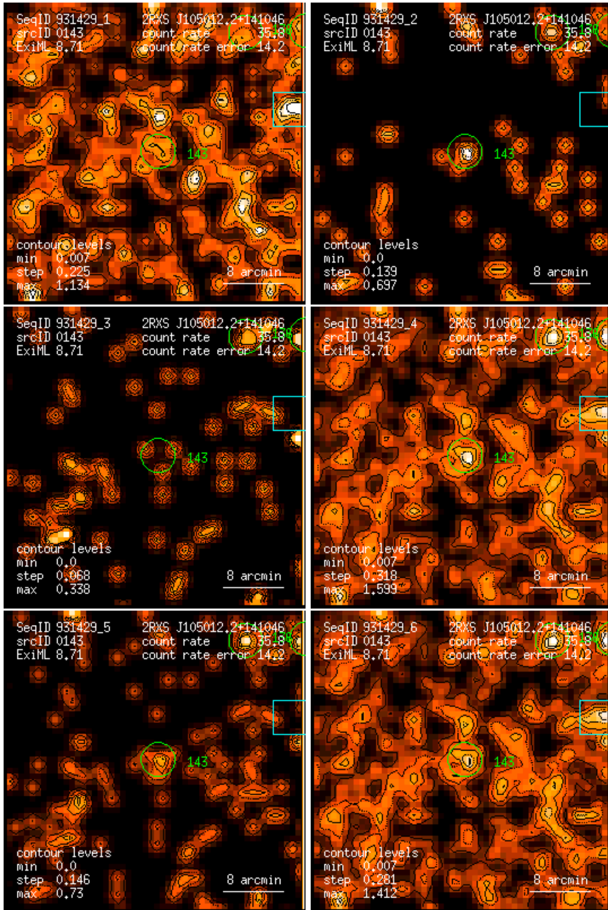
Figure 143: RASS 931429: detection 0143: band rate images, Gaussian filter: (1) PSPC channels 11 – 41, (2) 52 – 90, (3) 91 – 201, (4) 11 – 235, (5) 52 – 201, (6) 11 – 201. Broad band rates in counts/ks. Band rate contour levels in counts/ks/arcmin 2 .
