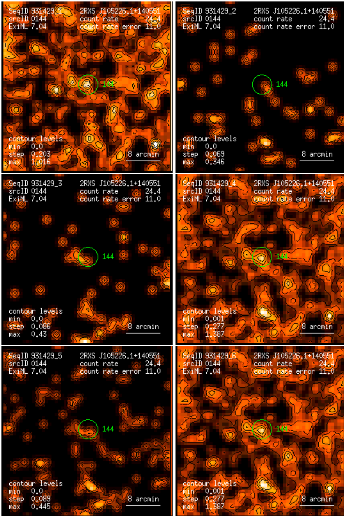
Figure 144: RASS 931429: detection 0144: band rate images, Gaussian filter: (1) PSPC channels 11 – 41, (2) 52 – 90, (3) 91 – 201, (4) 11 – 235, (5) 52 – 201, (6) 11 – 201. Broad band rates in counts/ks. Band rate contour levels in counts/ks/arcmin 2 .
