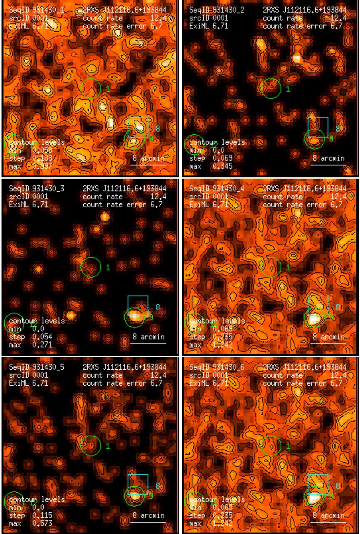
Figure 1: RASS 931430: detection 0001: band rate images, Gaussian filter: (1) PSPC channels 11 – 41, (2) 52 – 90, (3) 91 – 201, (4) 11 – 235, (5) 52 – 201, (6) 11 – 201. Broad band rates in counts/ks. Band rate contour levels in counts/ks/arcmin 2 .
