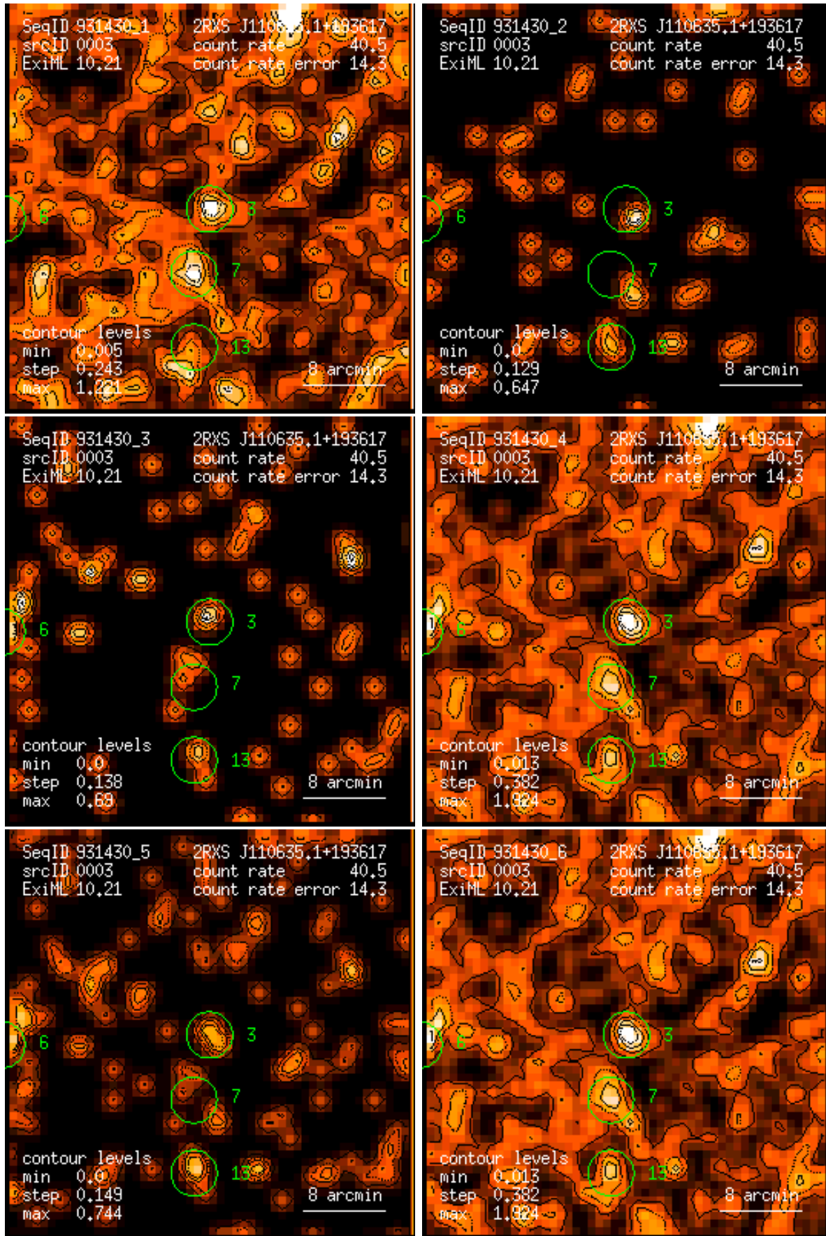
Figure 3: RASS 931430: detection 0003: band rate images, Gaussian filter: (1) PSPC channels 11 – 41, (2) 52 – 90, (3) 91 – 201, (4) 11 – 235, (5) 52 – 201, (6) 11 – 201. Broad band rates in counts/ks. Band rate contour levels in counts/ks/arcmin 2 .
