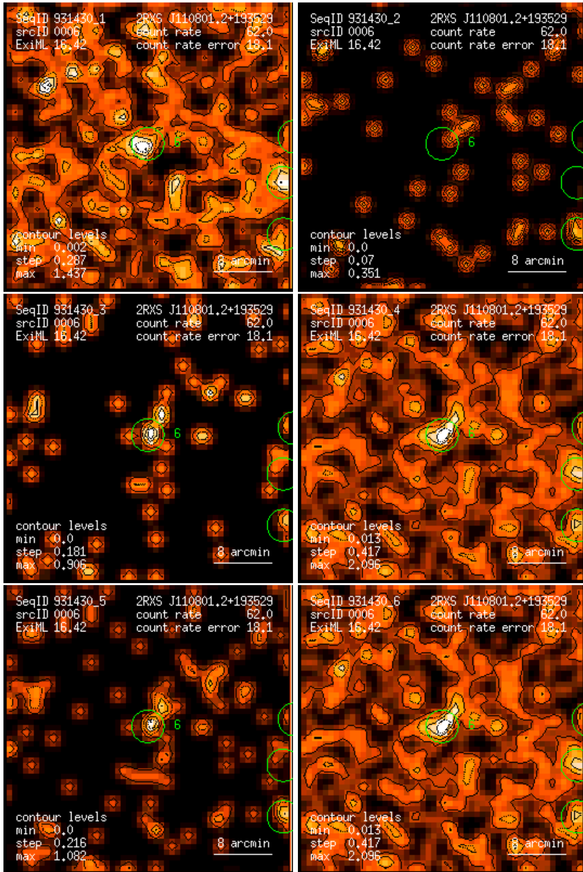
Figure 6: RASS 931430: detection 0006: band rate images, Gaussian filter: (1) PSPC channels 11 – 41, (2) 52 – 90, (3) 91 – 201, (4) 11 – 235, (5) 52 – 201, (6) 11 – 201. Broad band rates in counts/ks. Band rate contour levels in counts/ks/arcmin 2 .
