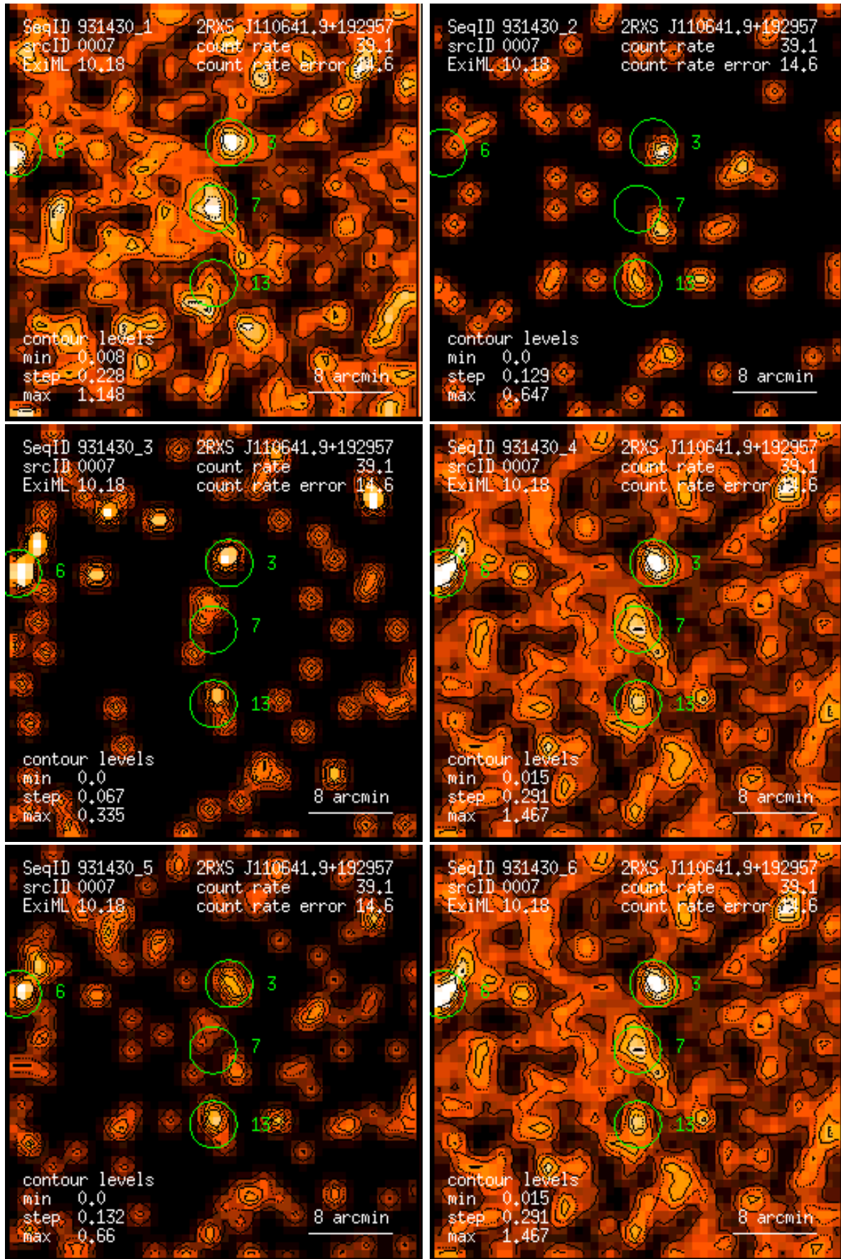
Figure 7: RASS 931430: detection 0007: band rate images, Gaussian filter: (1) PSPC channels 11 – 41, (2) 52 – 90, (3) 91 – 201, (4) 11 – 235, (5) 52 – 201, (6) 11 – 201. Broad band rates in counts/ks. Band rate contour levels in counts/ks/arcmin 2 .
