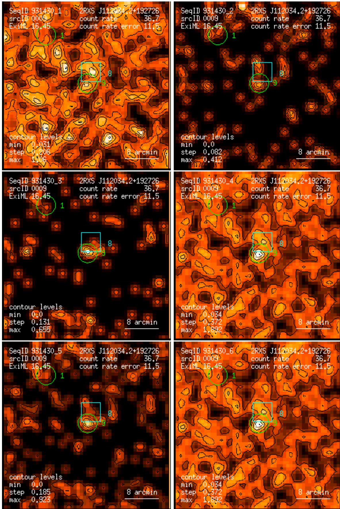
Figure 9: RASS 931430: detection 0009: band rate images, Gaussian filter: (1) PSPC channels 11 – 41, (2) 52 – 90, (3) 91 – 201, (4) 11 – 235, (5) 52 – 201, (6) 11 – 201. Broad band rates in counts/ks. Band rate contour levels in counts/ks/arcmin 2 .
