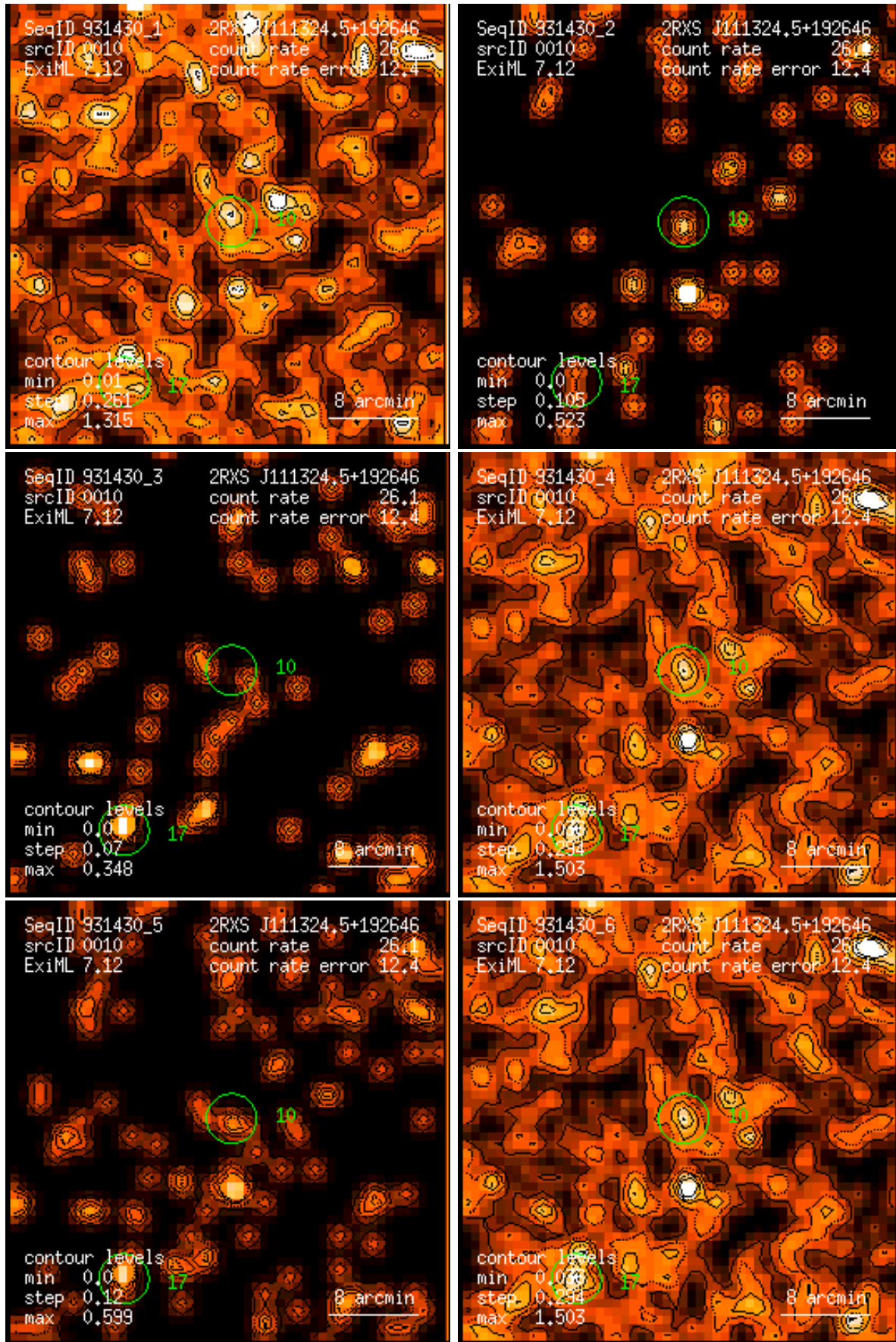
Figure 10: RASS 931430: detection 0010: band rate images, Gaussian filter: (1) PSPC channels 11 – 41, (2) 52 – 90, (3) 91 – 201, (4) 11 – 235, (5) 52 – 201, (6) 11 – 201. Broad band rates in counts/ks. Band rate contour levels in counts/ks/arcmin 2 .
