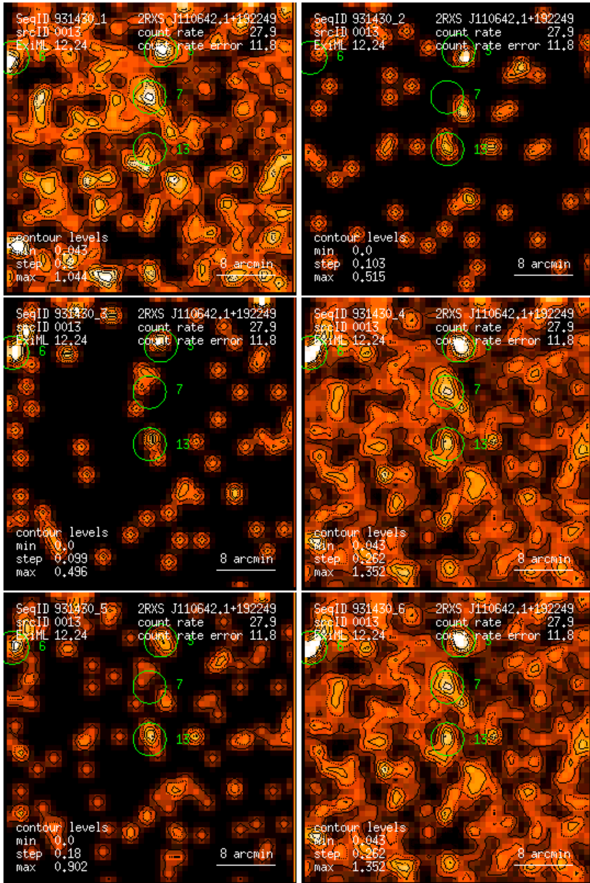
Figure 13: RASS 931430: detection 0013: band rate images, Gaussian filter: (1) PSPC channels 11 – 41, (2) 52 – 90, (3) 91 – 201, (4) 11 – 235, (5) 52 – 201, (6) 11 – 201. Broad band rates in counts/ks. Band rate contour levels in counts/ks/arcmin 2 .
