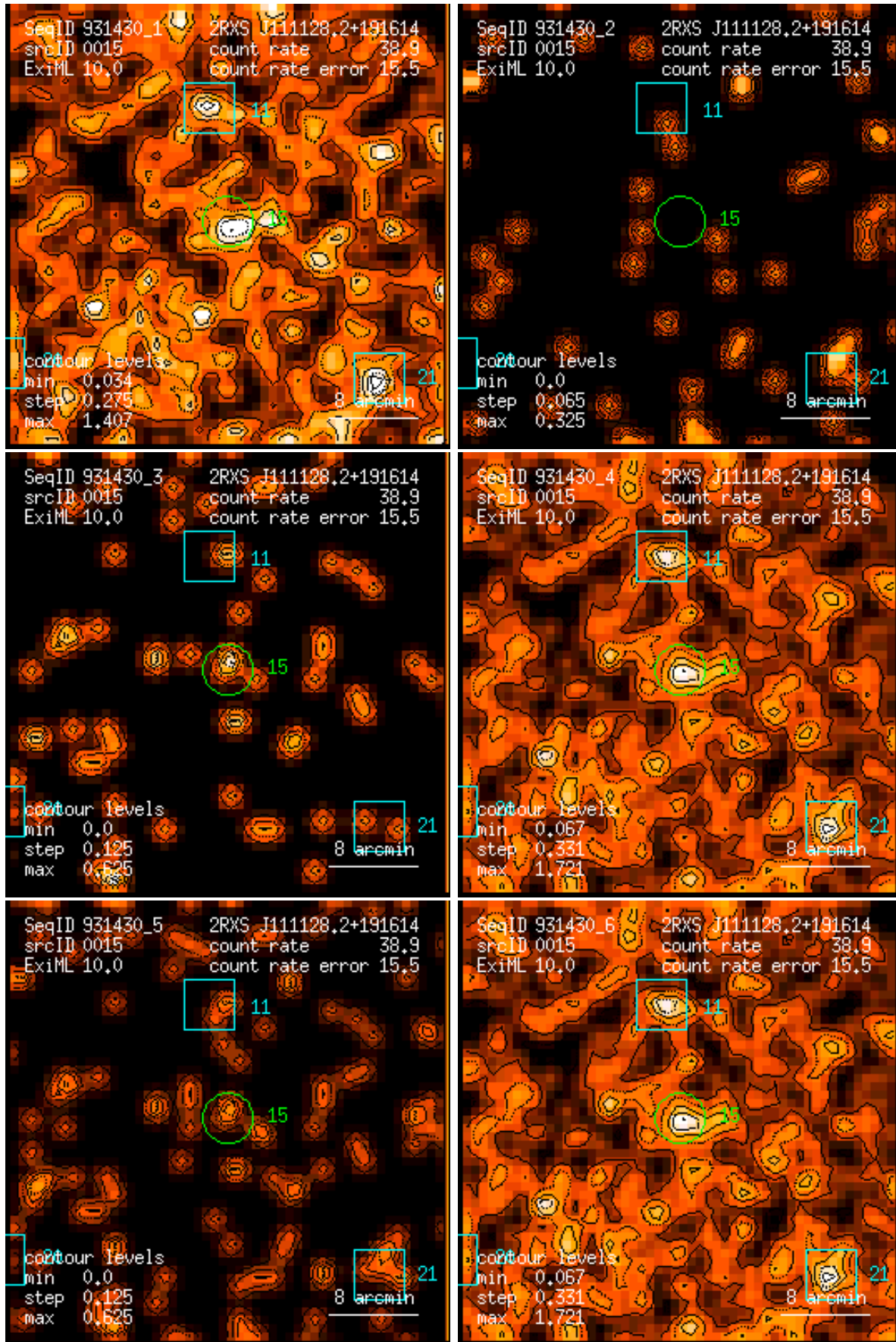
Figure 15: RASS 931430: detection 0015: band rate images, Gaussian filter: (1) PSPC channels 11 – 41, (2) 52 – 90, (3) 91 – 201, (4) 11 – 235, (5) 52 – 201, (6) 11 – 201. Broad band rates in counts/ks. Band rate contour levels in counts/ks/arcmin 2 .
