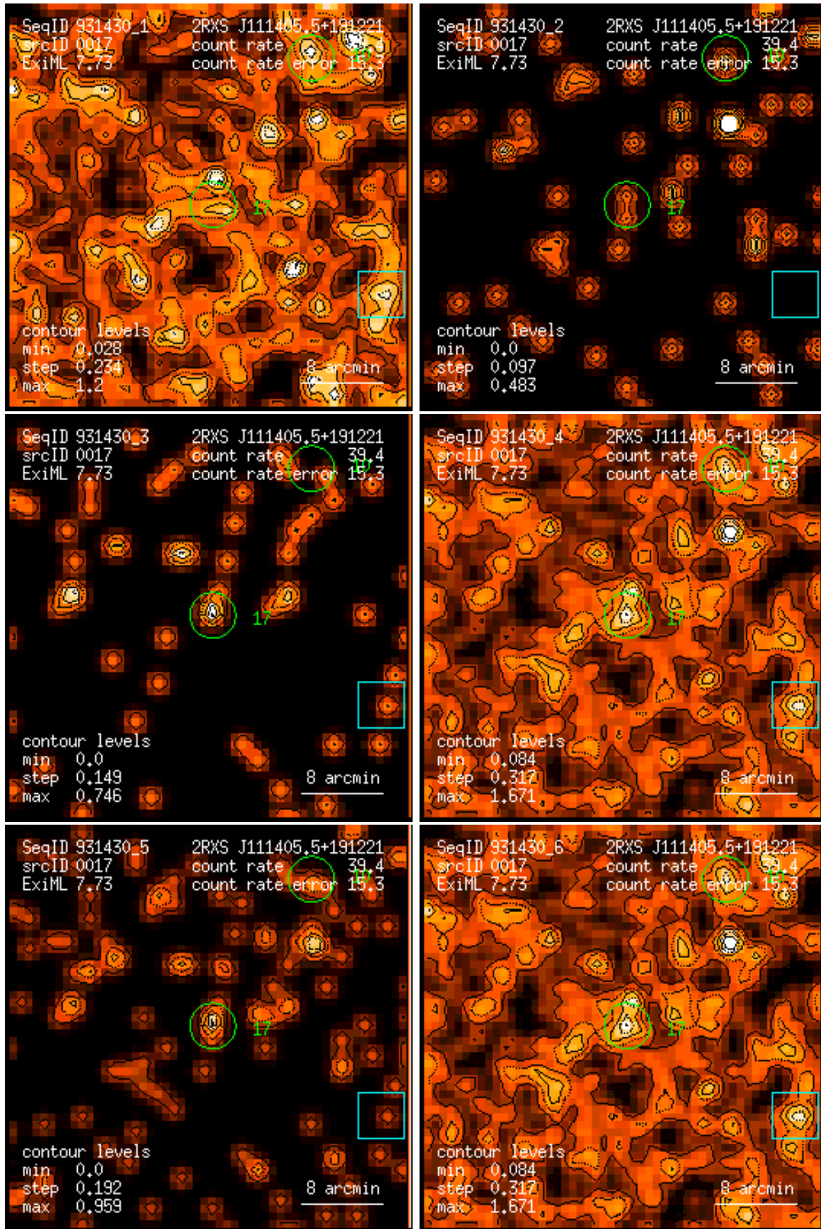
Figure 17: RASS 931430: detection 0017: band rate images, Gaussian filter: (1) PSPC channels 11 – 41, (2) 52 – 90, (3) 91 – 201, (4) 11 – 235, (5) 52 – 201, (6) 11 – 201. Broad band rates in counts/ks. Band rate contour levels in counts/ks/arcmin 2 .
