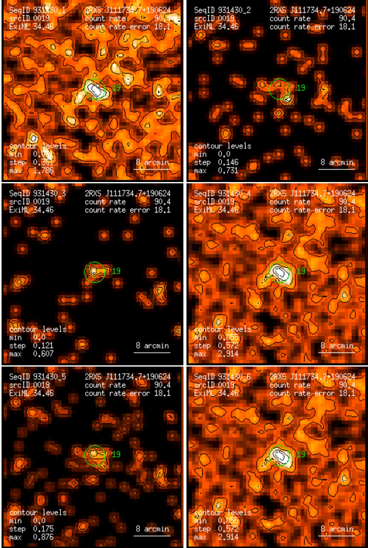
Figure 19: RASS 931430: detection 0019: band rate images, Gaussian filter: (1) PSPC channels 11 – 41, (2) 52 – 90, (3) 91 – 201, (4) 11 – 235, (5) 52 – 201, (6) 11 – 201. Broad band rates in counts/ks. Band rate contour levels in counts/ks/arcmin 2 .
