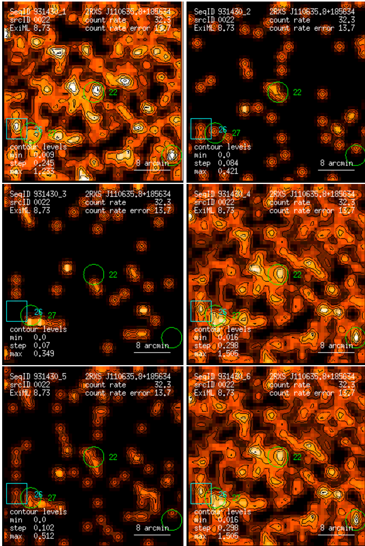
Figure 22: RASS 931430: detection 0022: band rate images, Gaussian filter: (1) PSPC channels 11 – 41, (2) 52 – 90, (3) 91 – 201, (4) 11 – 235, (5) 52 – 201, (6) 11 – 201. Broad band rates in counts/ks. Band rate contour levels in counts/ks/arcmin 2 .
