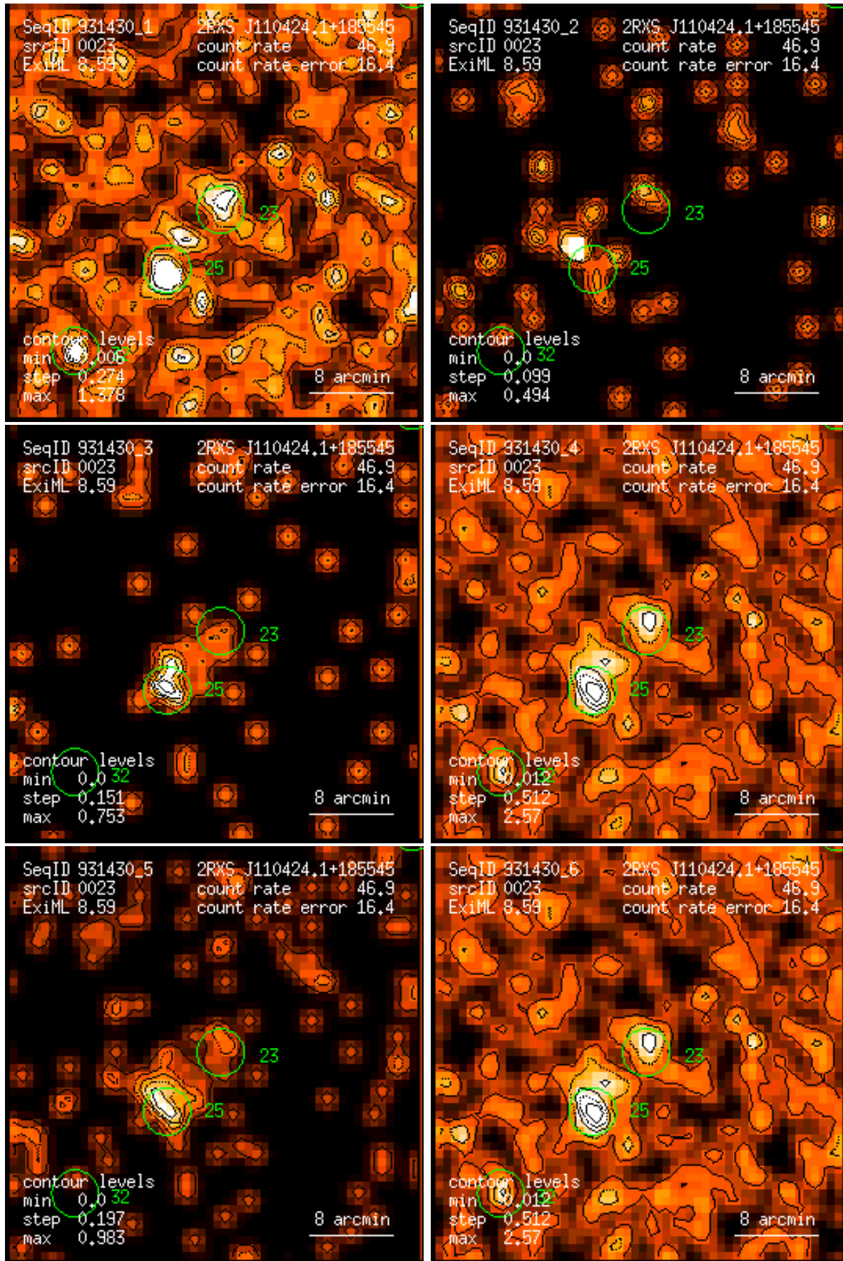
Figure 23: RASS 931430: detection 0023: band rate images, Gaussian filter: (1) PSPC channels 11 – 41, (2) 52 – 90, (3) 91 – 201, (4) 11 – 235, (5) 52 – 201, (6) 11 – 201. Broad band rates in counts/ks. Band rate contour levels in counts/ks/arcmin 2 .
