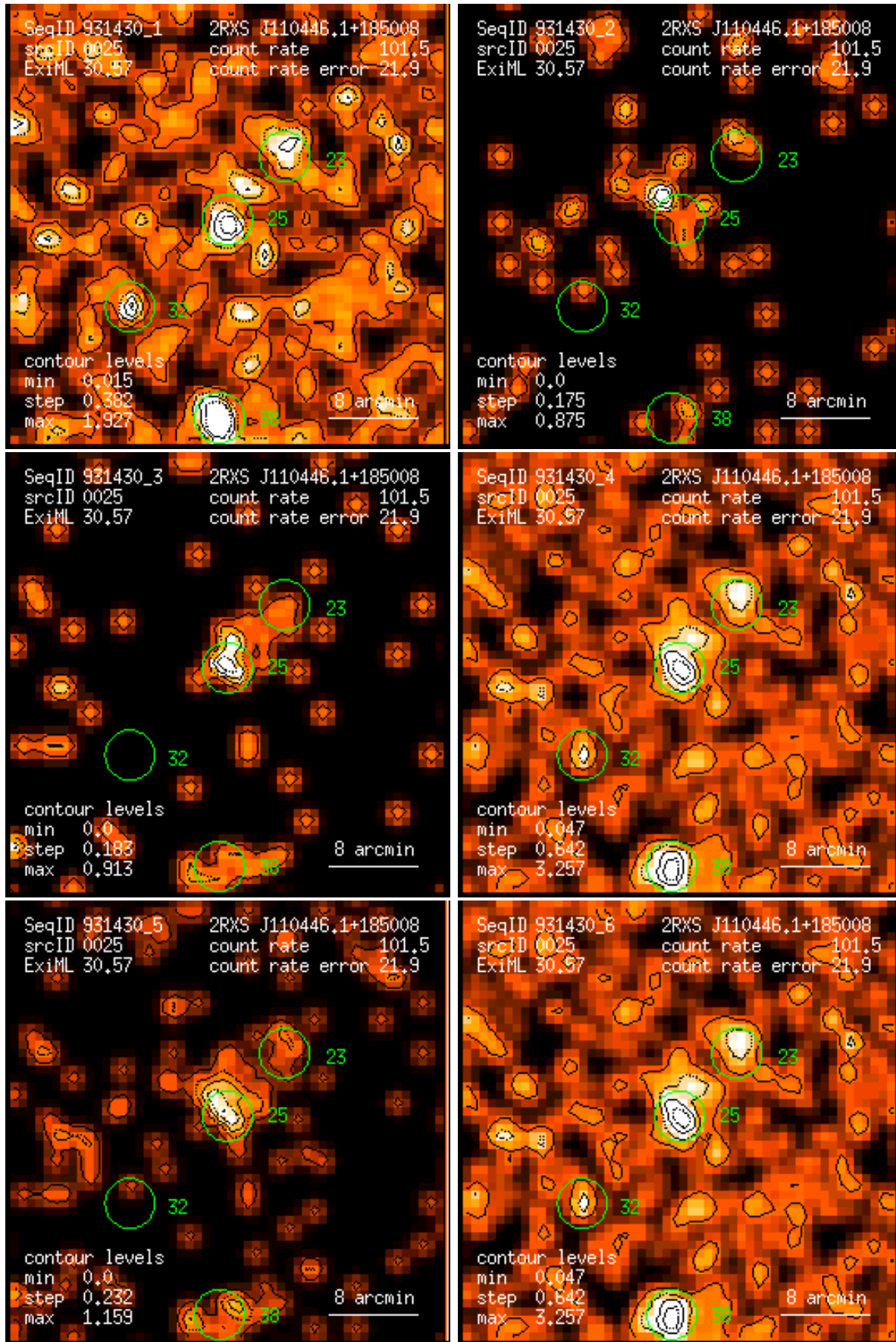
Figure 25: RASS 931430: detection 0025: band rate images, Gaussian filter: (1) PSPC channels 11 – 41, (2) 52 – 90, (3) 91 – 201, (4) 11 – 235, (5) 52 – 201, (6) 11 – 201. Broad band rates in counts/ks. Band rate contour levels in counts/ks/arcmin 2 .
