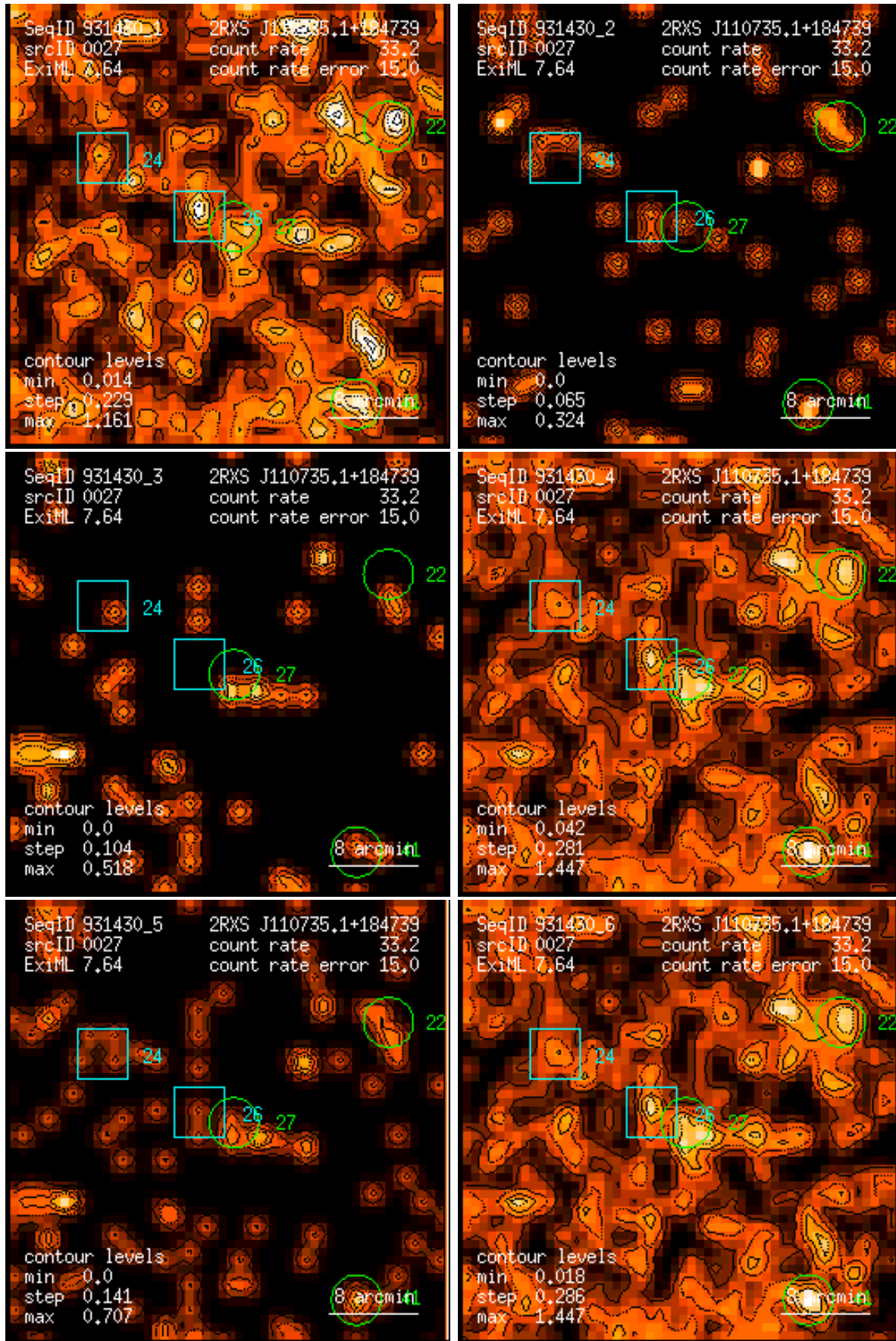
Figure 27: RASS 931430: detection 0027: band rate images, Gaussian filter: (1) PSPC channels 11 – 41, (2) 52 – 90, (3) 91 – 201, (4) 11 – 235, (5) 52 – 201, (6) 11 – 201. Broad band rates in counts/ks. Band rate contour levels in counts/ks/arcmin 2 .
