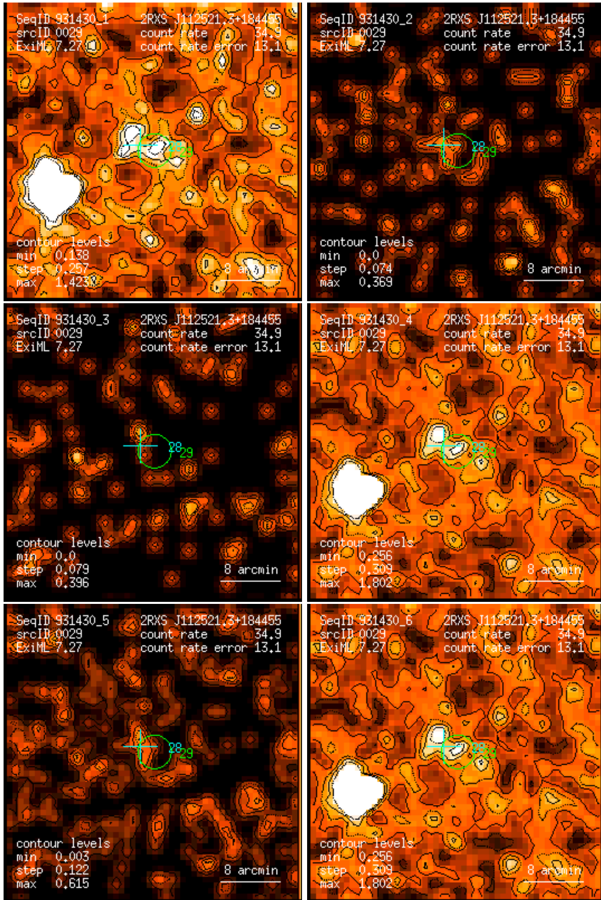
Figure 29: RASS 931430: detection 0029: band rate images, Gaussian filter: (1) PSPC channels 11 – 41, (2) 52 – 90, (3) 91 – 201, (4) 11 – 235, (5) 52 – 201, (6) 11 – 201. Broad band rates in counts/ks. Band rate contour levels in counts/ks/arcmin 2 .
