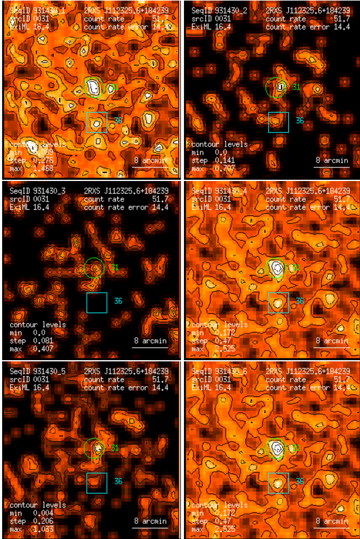
Figure 31: RASS 931430: detection 0031: band rate images, Gaussian filter: (1) PSPC channels 11 – 41, (2) 52 – 90, (3) 91 – 201, (4) 11 – 235, (5) 52 – 201, (6) 11 – 201. Broad band rates in counts/ks. Band rate contour levels in counts/ks/arcmin 2 .
