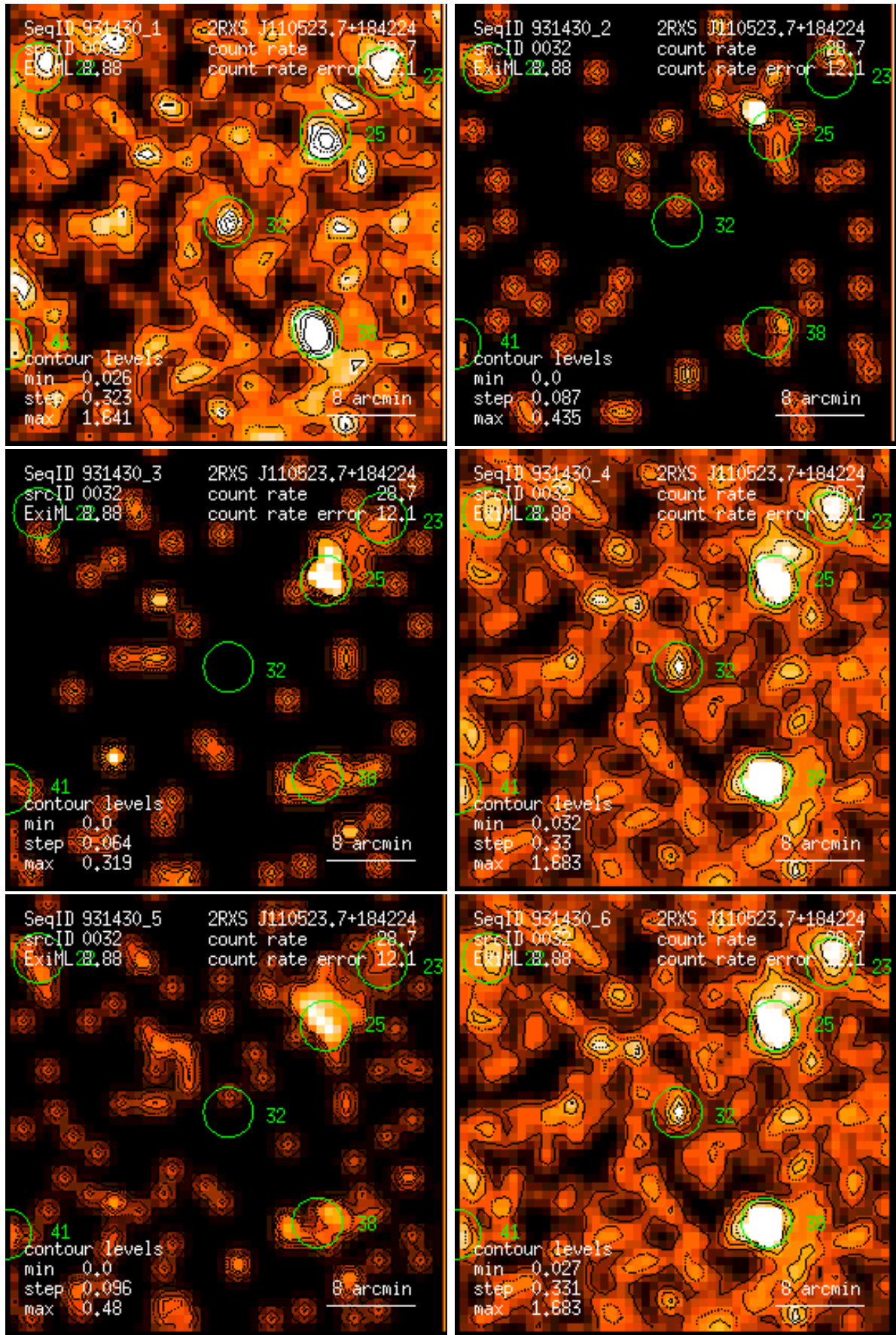
Figure 32: RASS 931430: detection 0032: band rate images, Gaussian filter: (1) PSPC channels 11 – 41, (2) 52 – 90, (3) 91 – 201, (4) 11 – 235, (5) 52 – 201, (6) 11 – 201. Broad band rates in counts/ks. Band rate contour levels in counts/ks/arcmin 2 .
