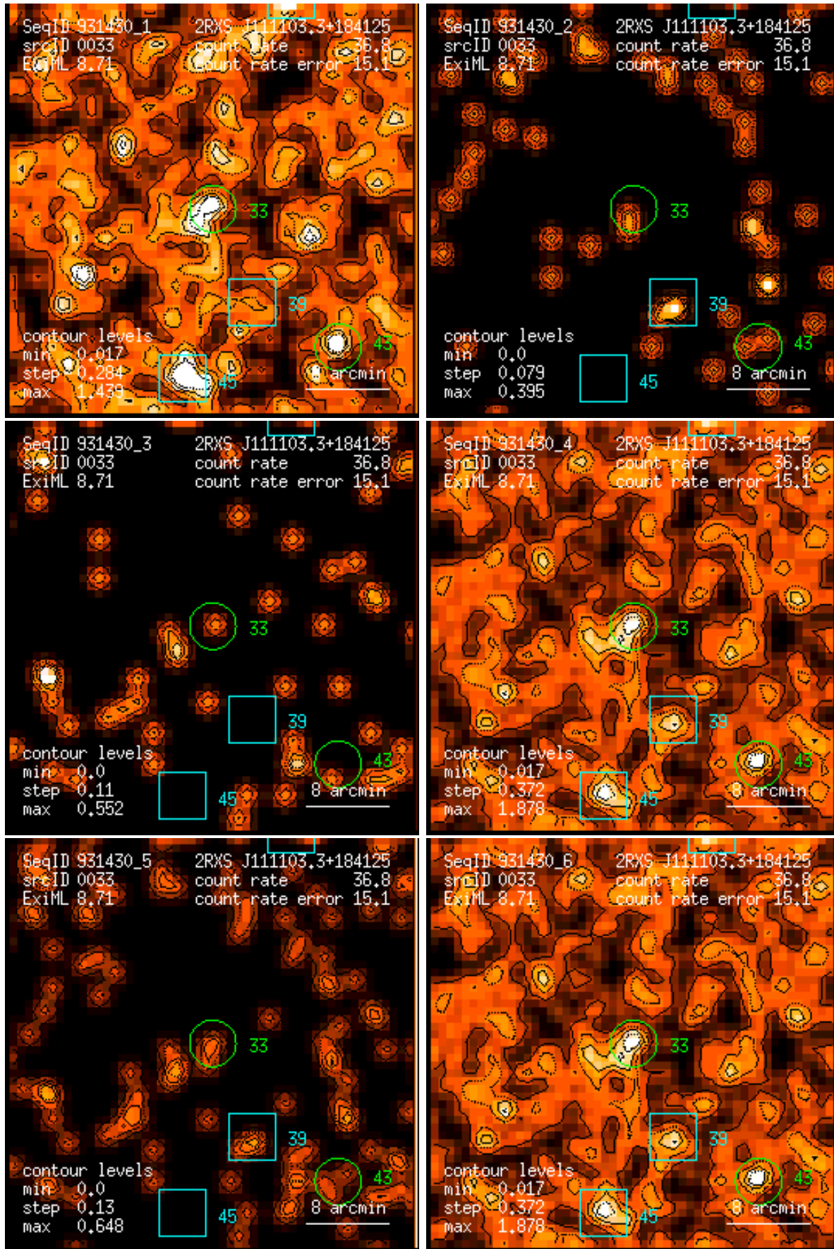
Figure 33: RASS 931430: detection 0033: band rate images, Gaussian filter: (1) PSPC channels 11 – 41, (2) 52 – 90, (3) 91 – 201, (4) 11 – 235, (5) 52 – 201, (6) 11 – 201. Broad band rates in counts/ks. Band rate contour levels in counts/ks/arcmin 2 .
