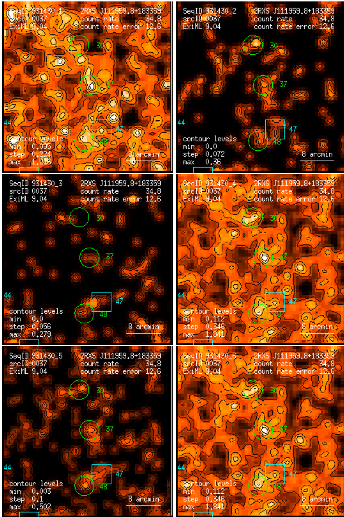
Figure 37: RASS 931430: detection 0037: band rate images, Gaussian filter: (1) PSPC channels 11 – 41, (2) 52 – 90, (3) 91 – 201, (4) 11 – 235, (5) 52 – 201, (6) 11 – 201. Broad band rates in counts/ks. Band rate contour levels in counts/ks/arcmin 2 .
