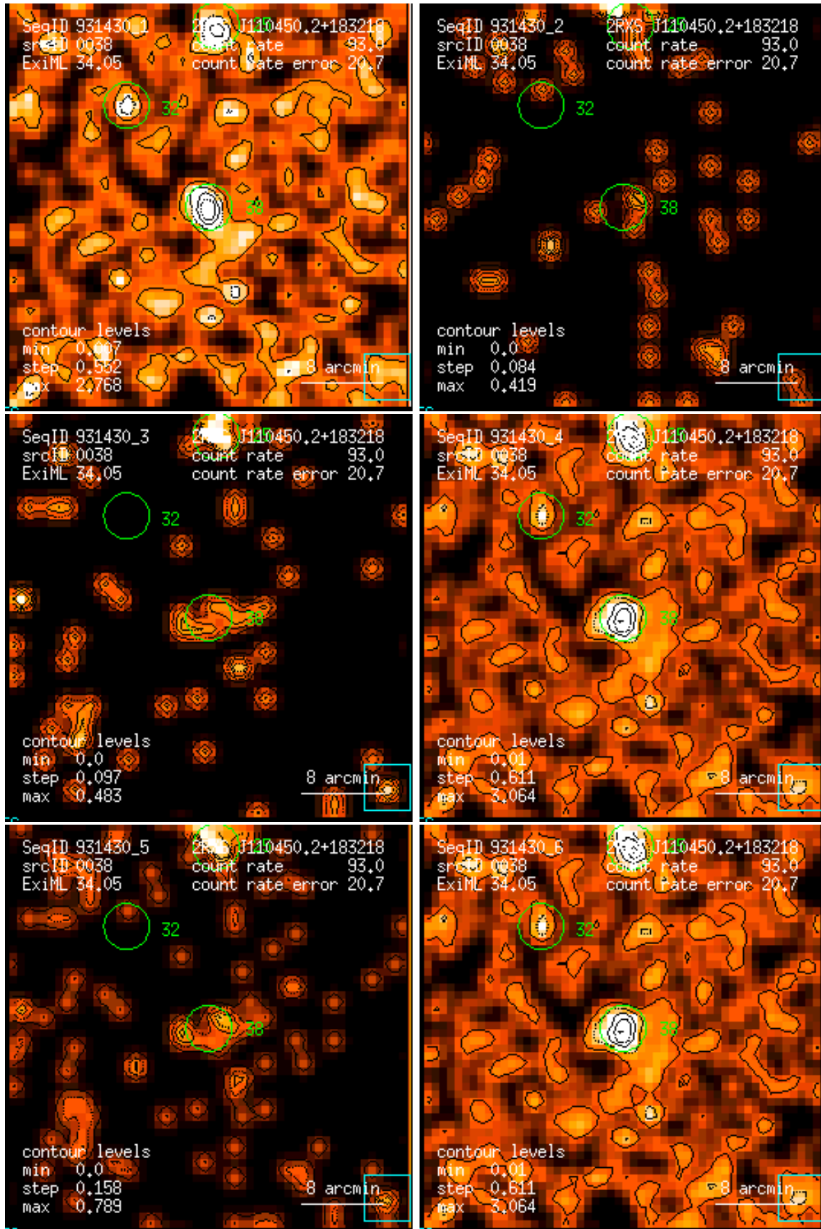
Figure 38: RASS 931430: detection 0038: band rate images, Gaussian filter: (1) PSPC channels 11 – 41, (2) 52 – 90, (3) 91 – 201, (4) 11 – 235, (5) 52 – 201, (6) 11 – 201. Broad band rates in counts/ks. Band rate contour levels in counts/ks/arcmin 2 .
