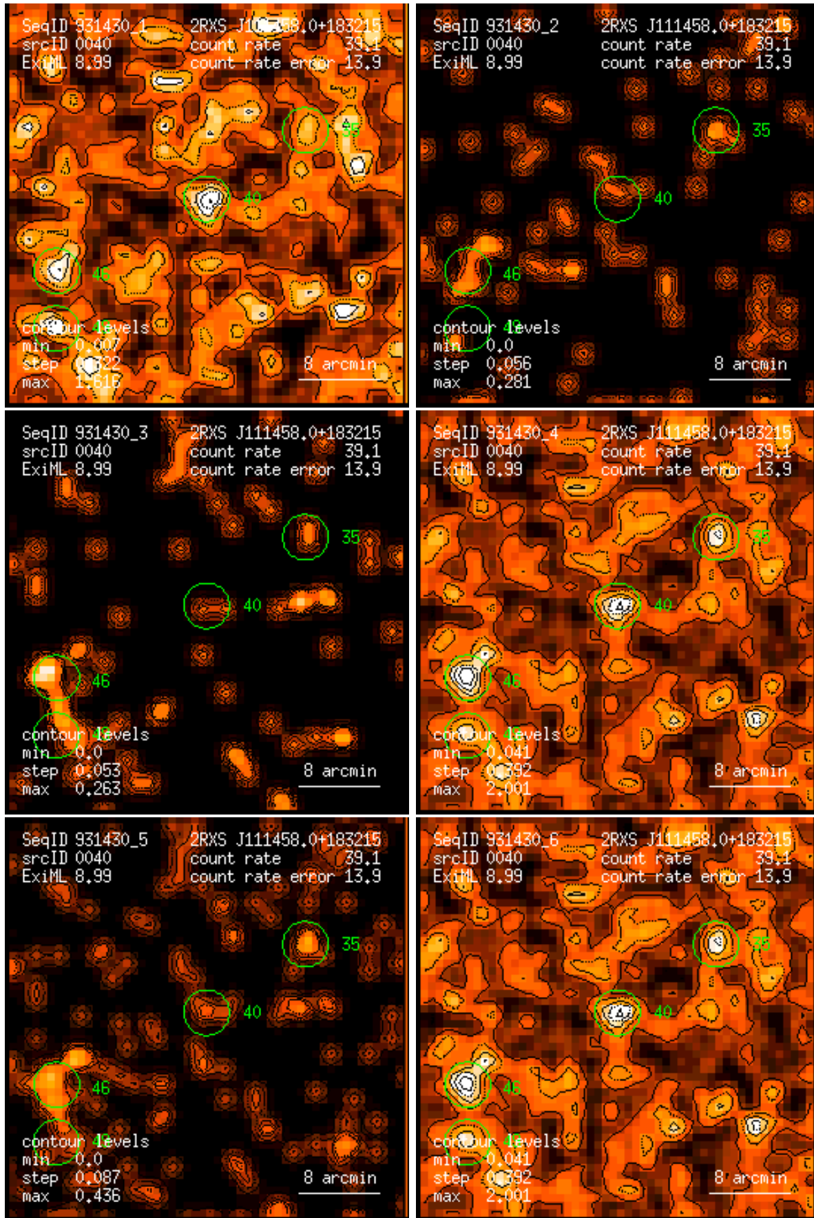
Figure 40: RASS 931430: detection 0040: band rate images, Gaussian filter: (1) PSPC channels 11 – 41, (2) 52 – 90, (3) 91 – 201, (4) 11 – 235, (5) 52 – 201, (6) 11 – 201. Broad band rates in counts/ks. Band rate contour levels in counts/ks/arcmin 2 .
