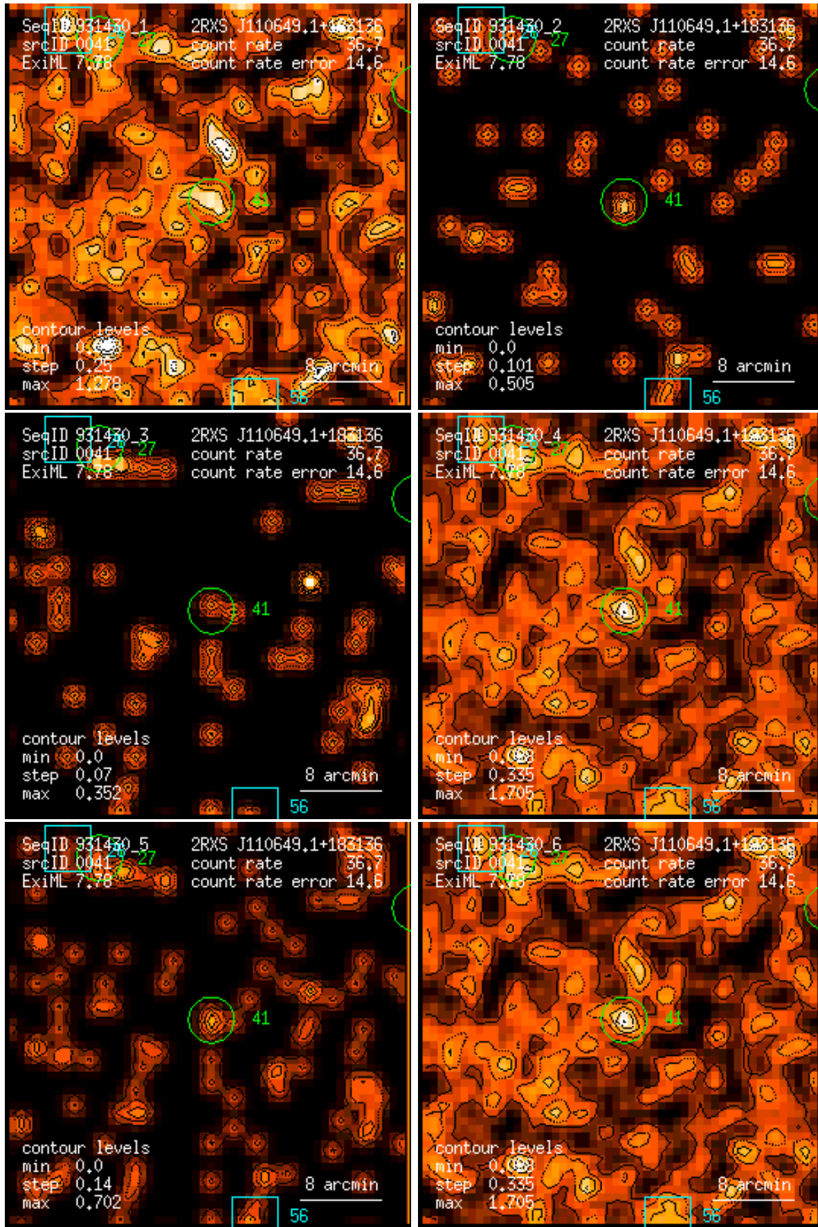
Figure 41: RASS 931430: detection 0041: band rate images, Gaussian filter: (1) PSPC channels 11 – 41, (2) 52 – 90, (3) 91 – 201, (4) 11 – 235, (5) 52 – 201, (6) 11 – 201. Broad band rates in counts/ks. Band rate contour levels in counts/ks/arcmin 2 .
