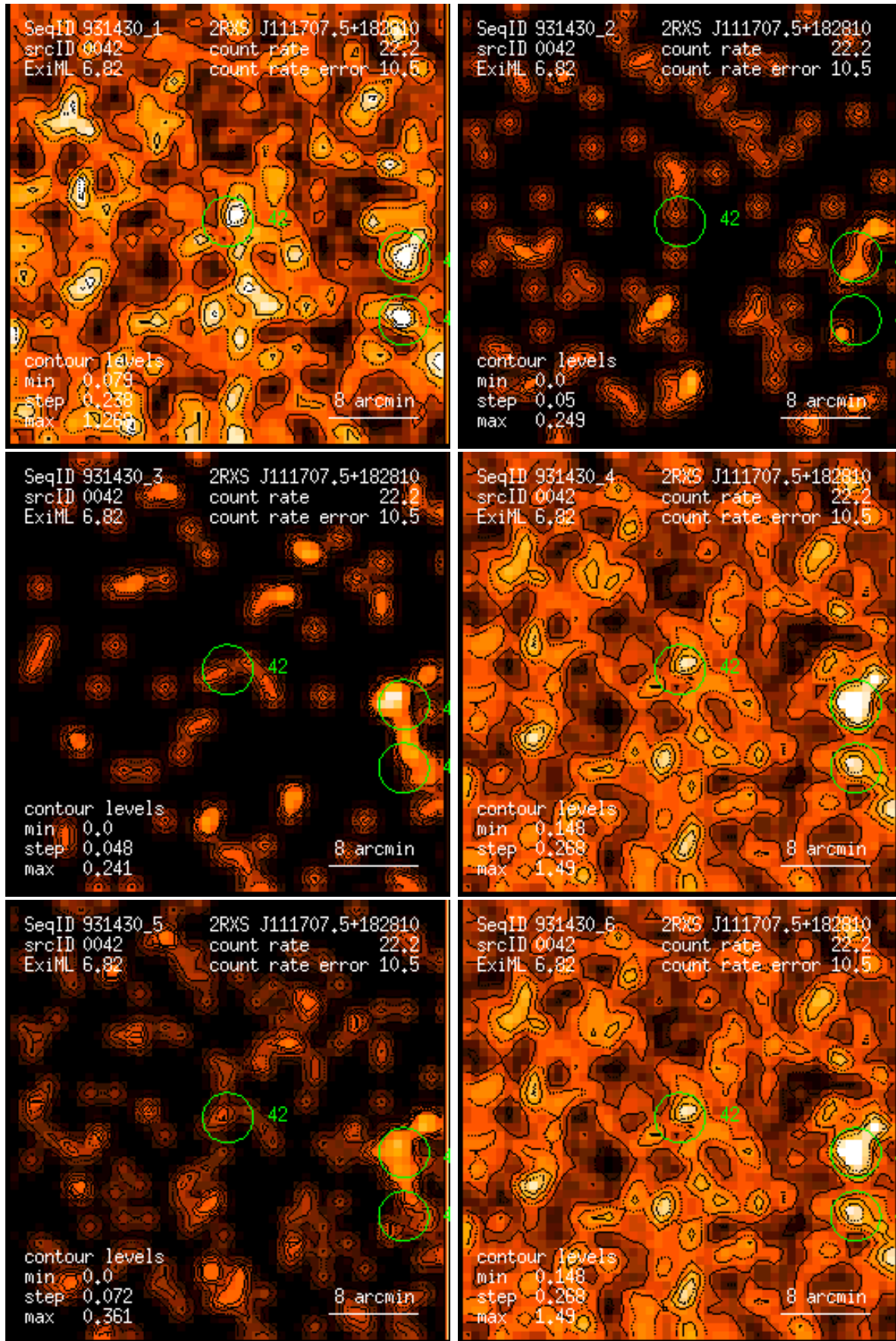
Figure 42: RASS 931430: detection 0042: band rate images, Gaussian filter: (1) PSPC channels 11 – 41, (2) 52 – 90, (3) 91 – 201, (4) 11 – 235, (5) 52 – 201, (6) 11 – 201. Broad band rates in counts/ks. Band rate contour levels in counts/ks/arcmin 2 .
