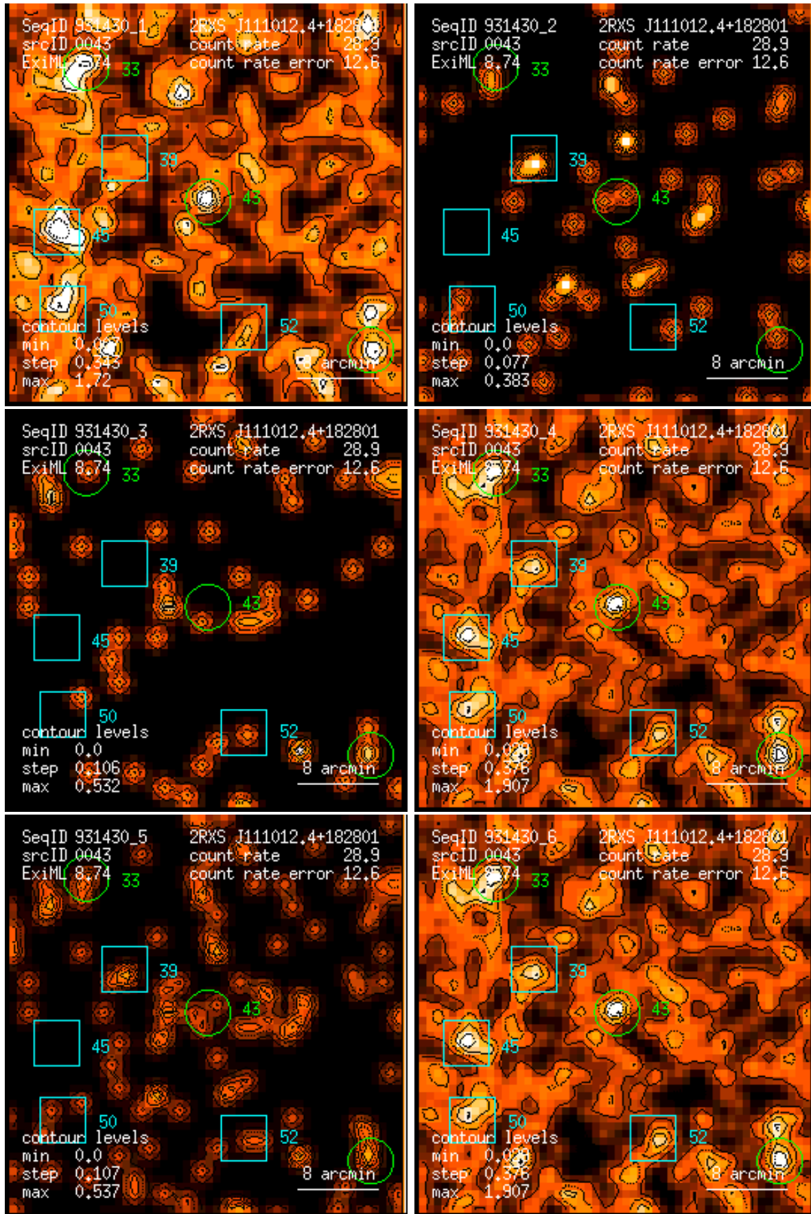
Figure 43: RASS 931430: detection 0043: band rate images, Gaussian filter: (1) PSPC channels 11 – 41, (2) 52 – 90, (3) 91 – 201, (4) 11 – 235, (5) 52 – 201, (6) 11 – 201. Broad band rates in counts/ks. Band rate contour levels in counts/ks/arcmin 2 .
