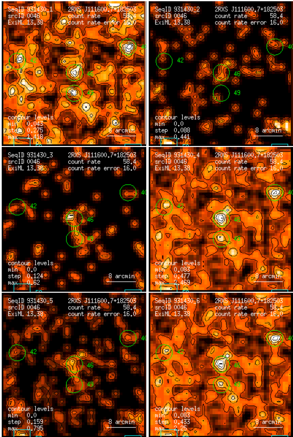
Figure 46: RASS 931430: detection 0046: band rate images, Gaussian filter: (1) PSPC channels 11 – 41, (2) 52 – 90, (3) 91 – 201, (4) 11 – 235, (5) 52 – 201, (6) 11 – 201. Broad band rates in counts/ks. Band rate contour levels in counts/ks/arcmin 2 .
