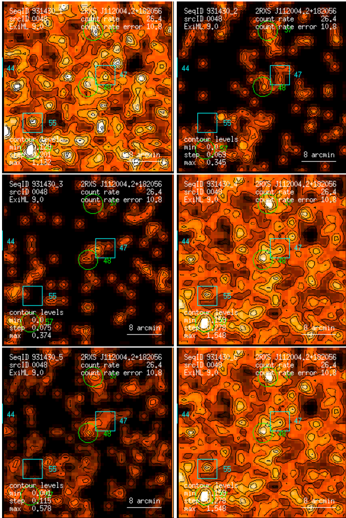
Figure 48: RASS 931430: detection 0048: band rate images, Gaussian filter: (1) PSPC channels 11 – 41, (2) 52 – 90, (3) 91 – 201, (4) 11 – 235, (5) 52 – 201, (6) 11 – 201. Broad band rates in counts/ks. Band rate contour levels in counts/ks/arcmin 2 .
