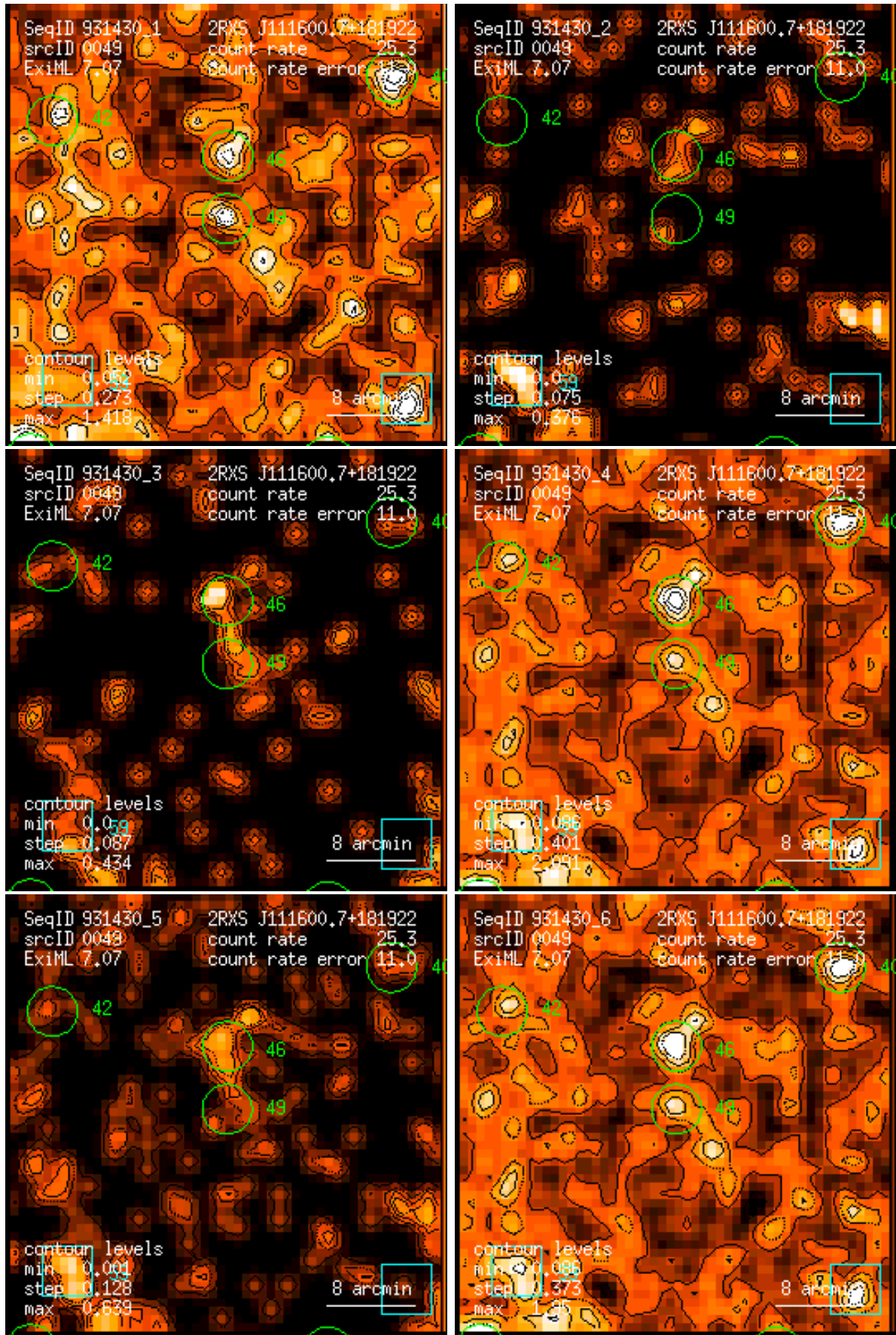
Figure 49: RASS 931430: detection 0049: band rate images, Gaussian filter: (1) PSPC channels 11 – 41, (2) 52 – 90, (3) 91 – 201, (4) 11 – 235, (5) 52 – 201, (6) 11 – 201. Broad band rates in counts/ks. Band rate contour levels in counts/ks/arcmin 2 .
