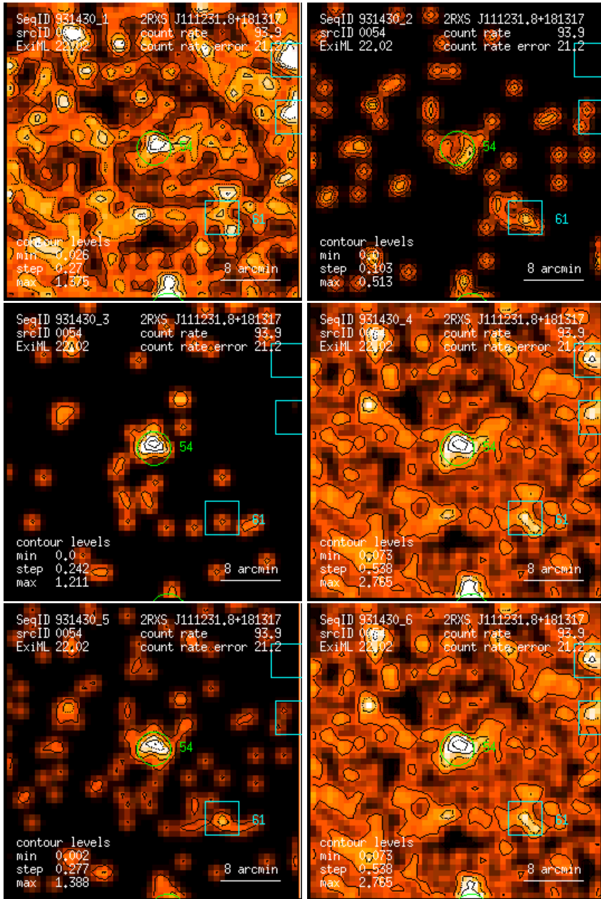
Figure 54: RASS 931430: detection 0054: band rate images, Gaussian filter: (1) PSPC channels 11 – 41, (2) 52 – 90, (3) 91 – 201, (4) 11 – 235, (5) 52 – 201, (6) 11 – 201. Broad band rates in counts/ks. Band rate contour levels in counts/ks/arcmin 2 .
