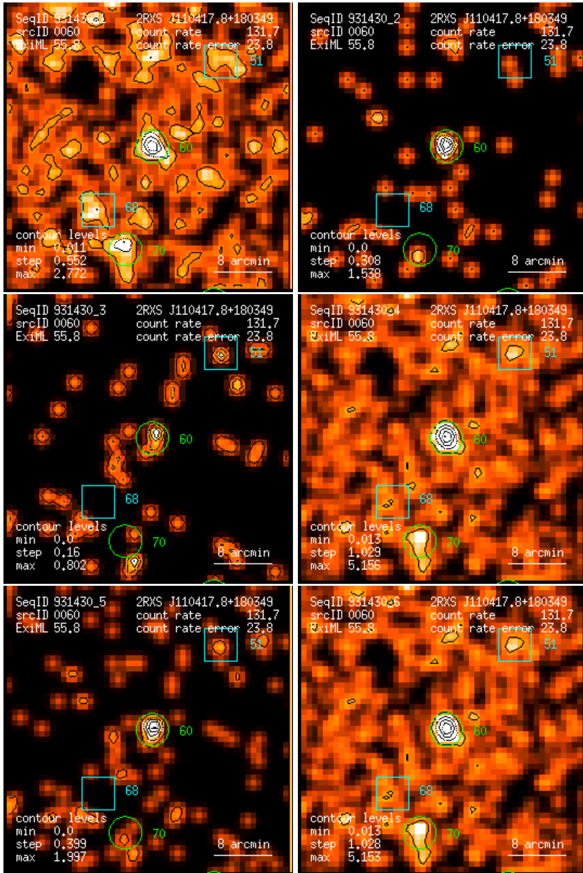
Figure 60: RASS 931430: detection 0060: band rate images, Gaussian filter: (1) PSPC channels 11 – 41, (2) 52 – 90, (3) 91 – 201, (4) 11 – 235, (5) 52 – 201, (6) 11 – 201. Broad band rates in counts/ks. Band rate contour levels in counts/ks/arcmin 2 .
