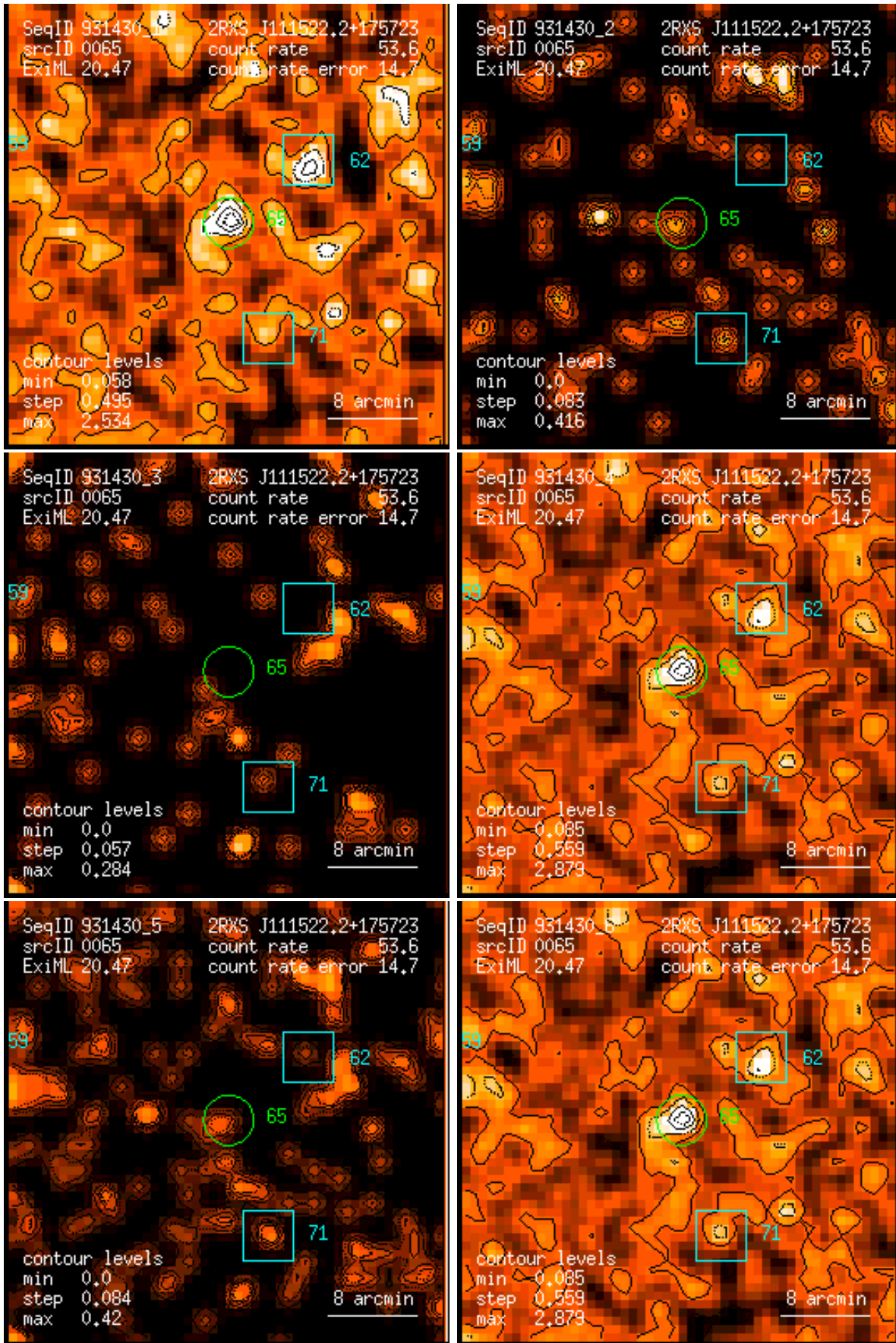
Figure 65: RASS 931430: detection 0065: band rate images, Gaussian filter: (1) PSPC channels 11 – 41, (2) 52 – 90, (3) 91 – 201, (4) 11 – 235, (5) 52 – 201, (6) 11 – 201. Broad band rates in counts/ks. Band rate contour levels in counts/ks/arcmin 2 .
