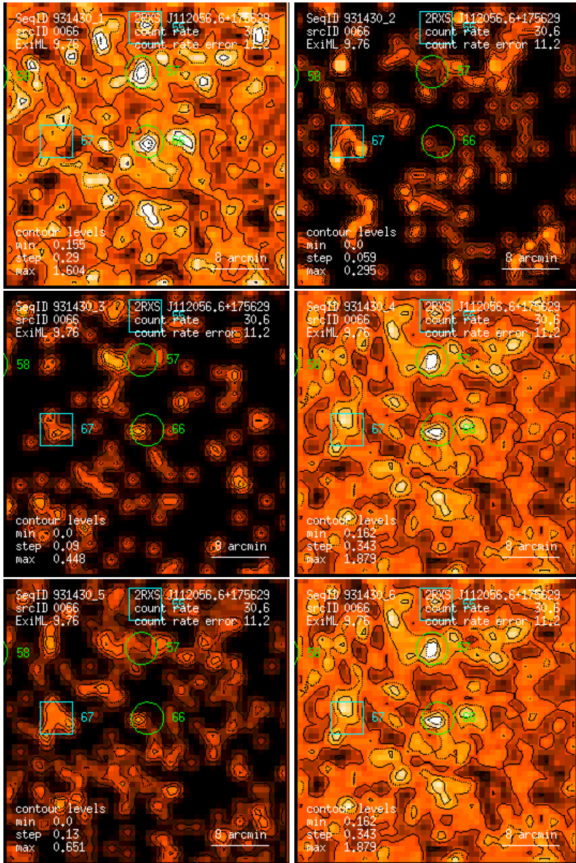
Figure 66: RASS 931430: detection 0066: band rate images, Gaussian filter: (1) PSPC channels 11 – 41, (2) 52 – 90, (3) 91 – 201, (4) 11 – 235, (5) 52 – 201, (6) 11 – 201. Broad band rates in counts/ks. Band rate contour levels in counts/ks/arcmin 2 .
