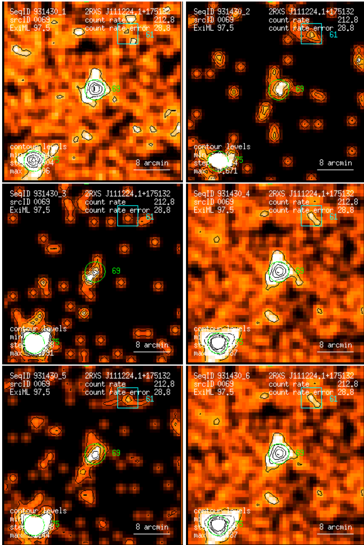
Figure 69: RASS 931430: detection 0069: band rate images, Gaussian filter: (1) PSPC channels 11 – 41, (2) 52 – 90, (3) 91 – 201, (4) 11 – 235, (5) 52 – 201, (6) 11 – 201. Broad band rates in counts/ks. Band rate contour levels in counts/ks/arcmin 2 .
