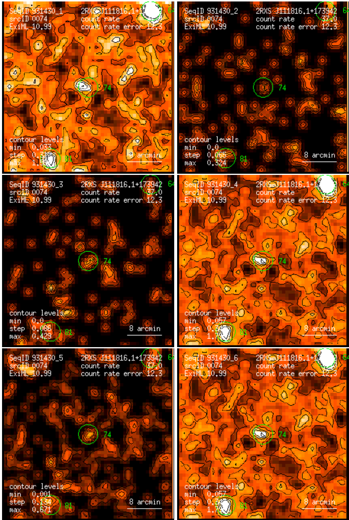
Figure 74: RASS 931430: detection 0074: band rate images, Gaussian filter: (1) PSPC channels 11 – 41, (2) 52 – 90, (3) 91 – 201, (4) 11 – 235, (5) 52 – 201, (6) 11 – 201. Broad band rates in counts/ks. Band rate contour levels in counts/ks/arcmin 2 .
