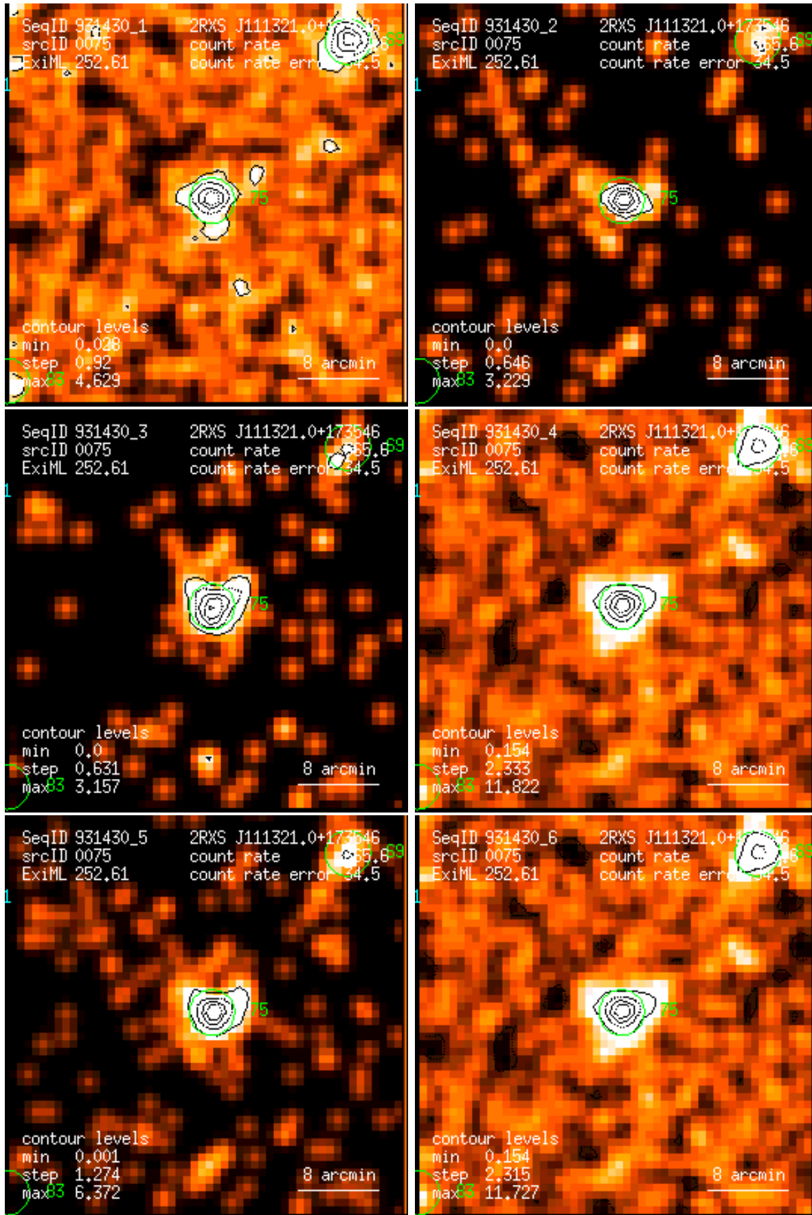
Figure 75: RASS 931430: detection 0075: band rate images, Gaussian filter: (1) PSPC channels 11 – 41, (2) 52 – 90, (3) 91 – 201, (4) 11 – 235, (5) 52 – 201, (6) 11 – 201. Broad band rates in counts/ks. Band rate contour levels in counts/ks/arcmin 2 .
