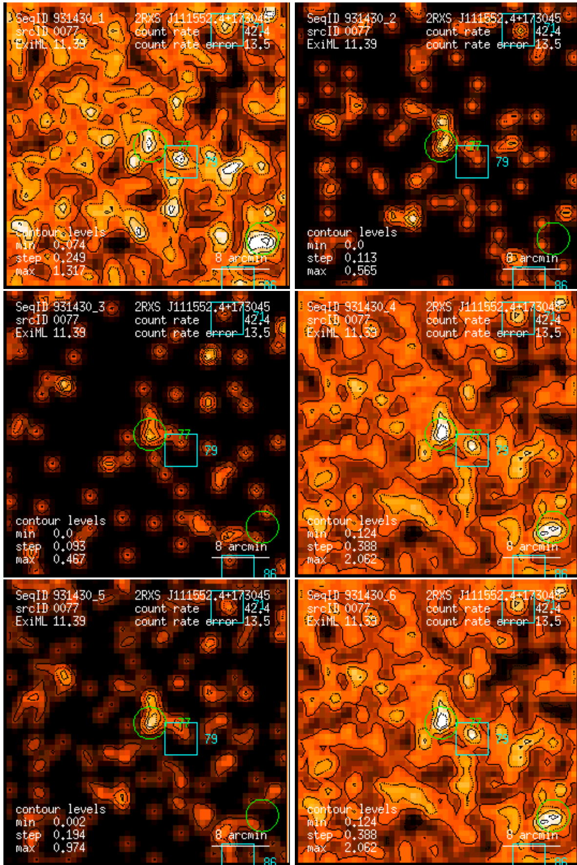
Figure 77: RASS 931430: detection 0077: band rate images, Gaussian filter: (1) PSPC channels 11 – 41, (2) 52 – 90, (3) 91 – 201, (4) 11 – 235, (5) 52 – 201, (6) 11 – 201. Broad band rates in counts/ks. Band rate contour levels in counts/ks/arcmin 2 .
