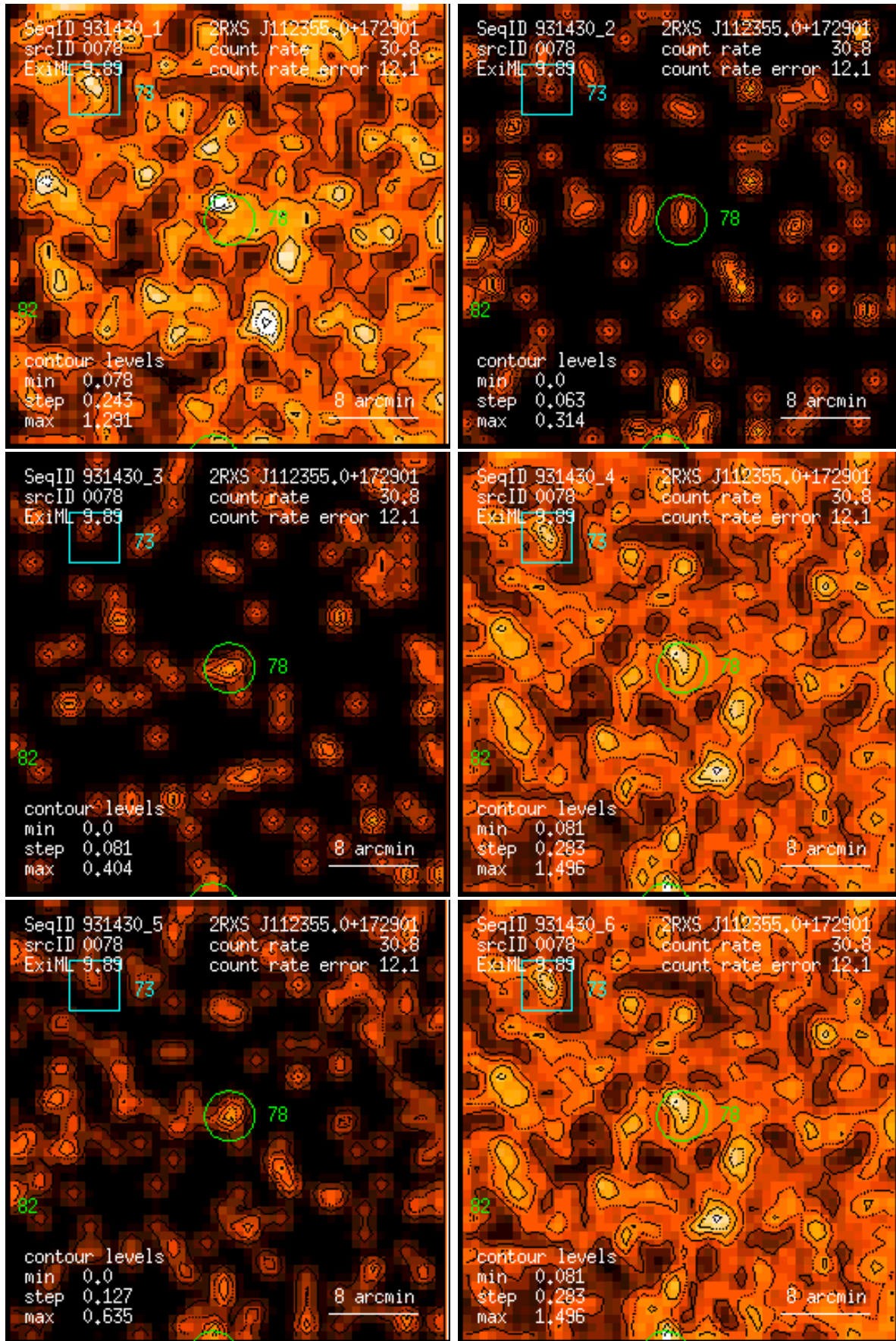
Figure 78: RASS 931430: detection 0078: band rate images, Gaussian filter: (1) PSPC channels 11 – 41, (2) 52 – 90, (3) 91 – 201, (4) 11 – 235, (5) 52 – 201, (6) 11 – 201. Broad band rates in counts/ks. Band rate contour levels in counts/ks/arcmin 2 .
