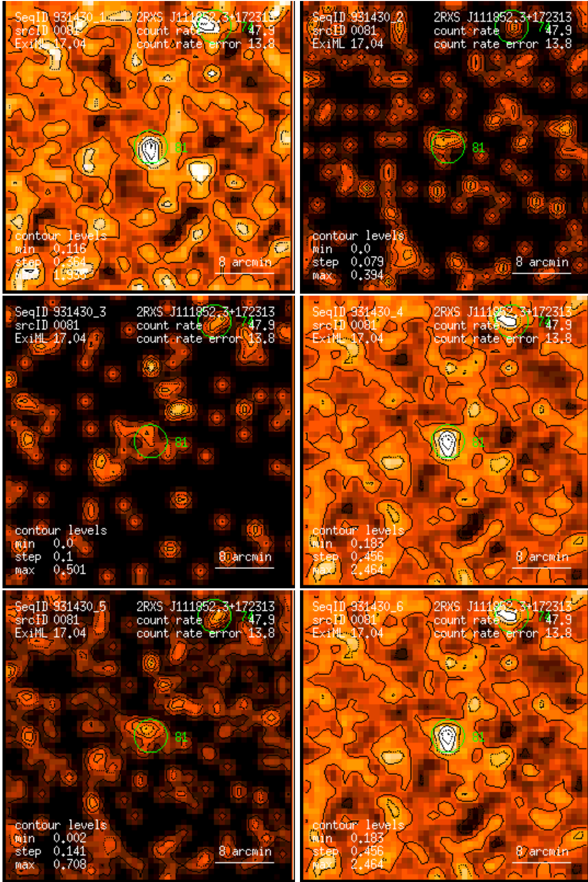
Figure 81: RASS 931430: detection 0081: band rate images, Gaussian filter: (1) PSPC channels 11 – 41, (2) 52 – 90, (3) 91 – 201, (4) 11 – 235, (5) 52 – 201, (6) 11 – 201. Broad band rates in counts/ks. Band rate contour levels in counts/ks/arcmin 2 .
