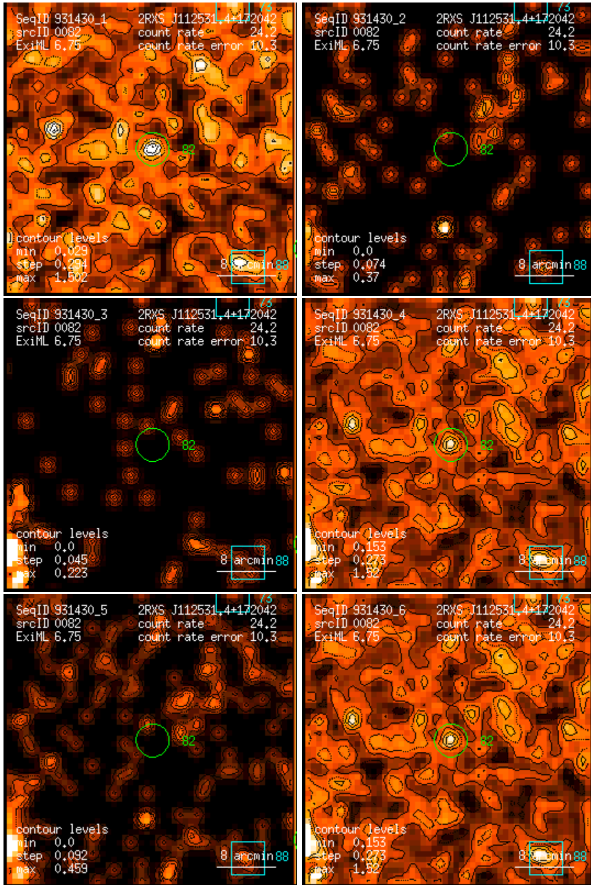
Figure 82: RASS 931430: detection 0082: band rate images, Gaussian filter: (1) PSPC channels 11 – 41, (2) 52 – 90, (3) 91 – 201, (4) 11 – 235, (5) 52 – 201, (6) 11 – 201. Broad band rates in counts/ks. Band rate contour levels in counts/ks/arcmin 2 .
