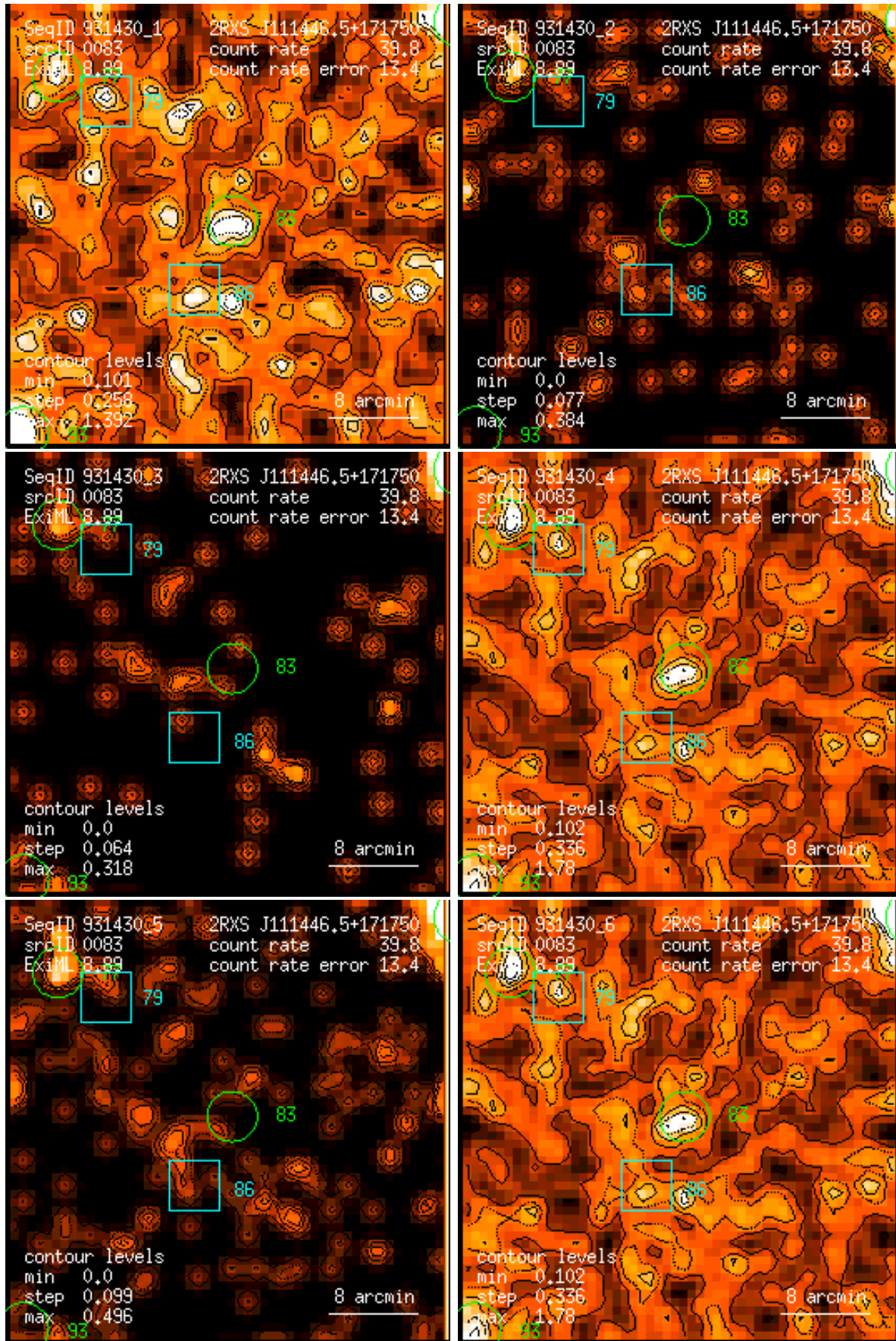
Figure 83: RASS 931430: detection 0083: band rate images, Gaussian filter: (1) PSPC channels 11 – 41, (2) 52 – 90, (3) 91 – 201, (4) 11 – 235, (5) 52 – 201, (6) 11 – 201. Broad band rates in counts/ks. Band rate contour levels in counts/ks/arcmin 2 .
