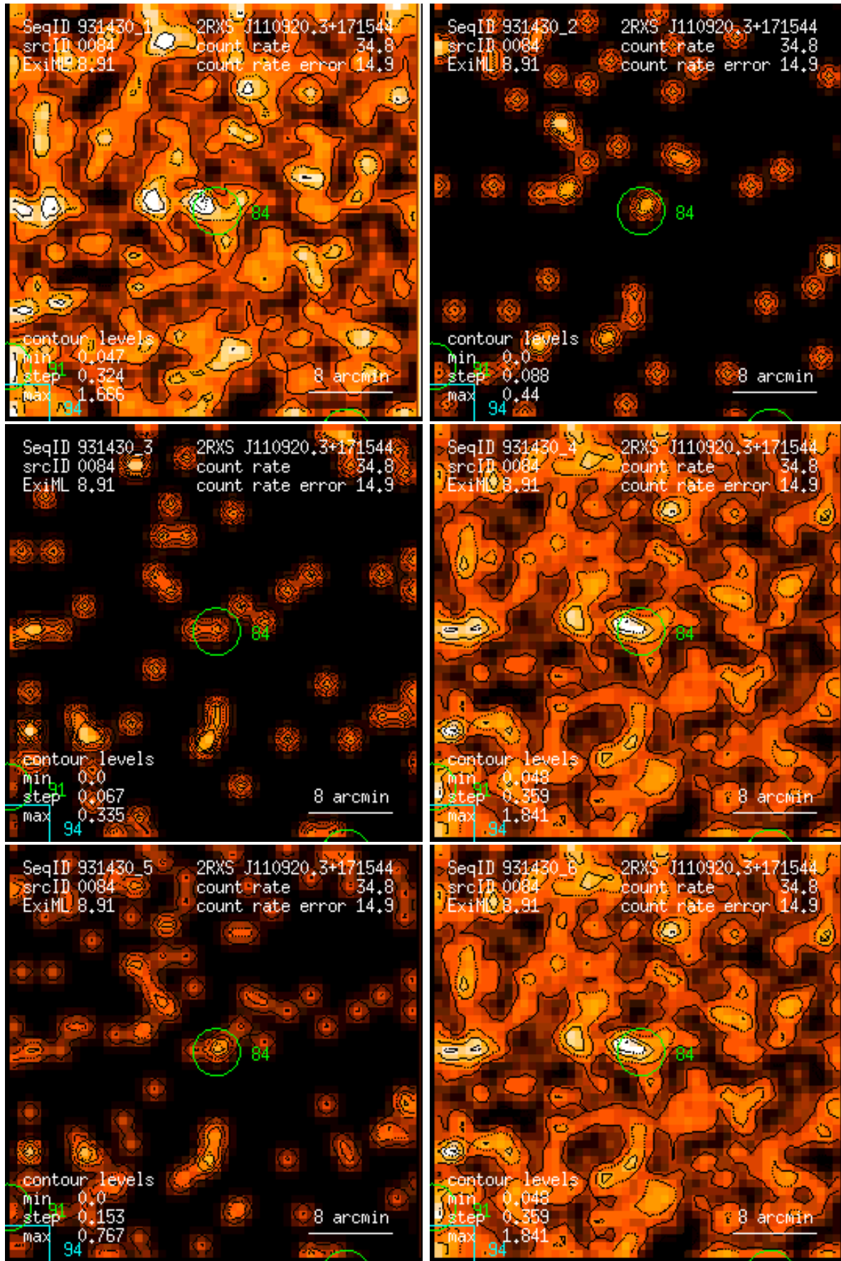
Figure 84: RASS 931430: detection 0084: band rate images, Gaussian filter: (1) PSPC channels 11 – 41, (2) 52 – 90, (3) 91 – 201, (4) 11 – 235, (5) 52 – 201, (6) 11 – 201. Broad band rates in counts/ks. Band rate contour levels in counts/ks/arcmin 2 .
