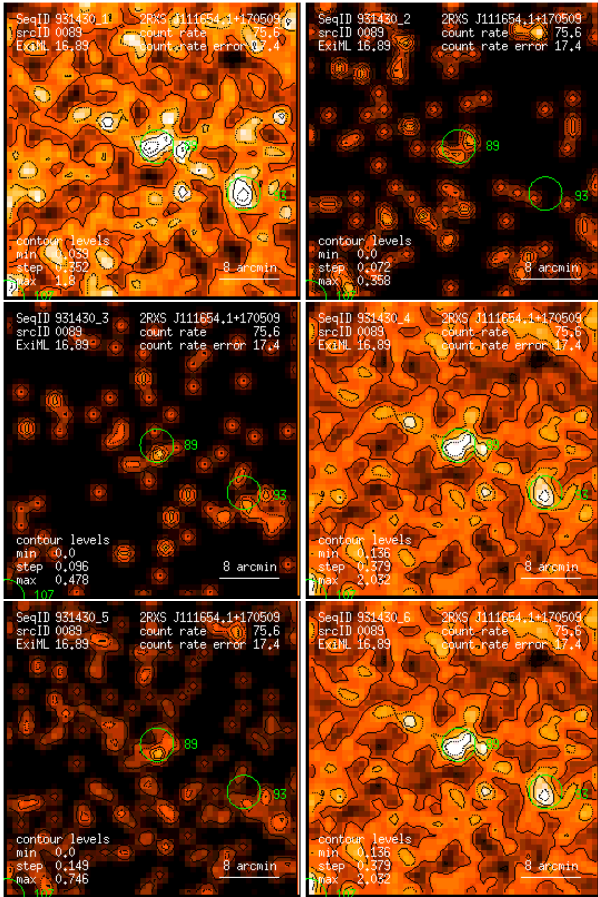
Figure 89: RASS 931430: detection 0089: band rate images, Gaussian filter: (1) PSPC channels 11 – 41, (2) 52 – 90, (3) 91 – 201, (4) 11 – 235, (5) 52 – 201, (6) 11 – 201. Broad band rates in counts/ks. Band rate contour levels in counts/ks/arcmin 2 .
