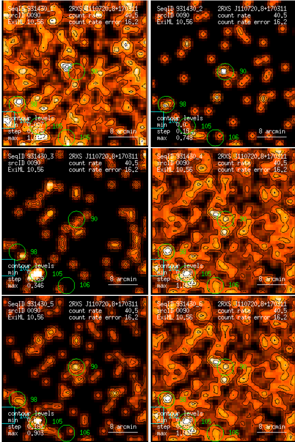
Figure 90: RASS 931430: detection 0090: band rate images, Gaussian filter: (1) PSPC channels 11 – 41, (2) 52 – 90, (3) 91 – 201, (4) 11 – 235, (5) 52 – 201, (6) 11 – 201. Broad band rates in counts/ks. Band rate contour levels in counts/ks/arcmin 2 .
