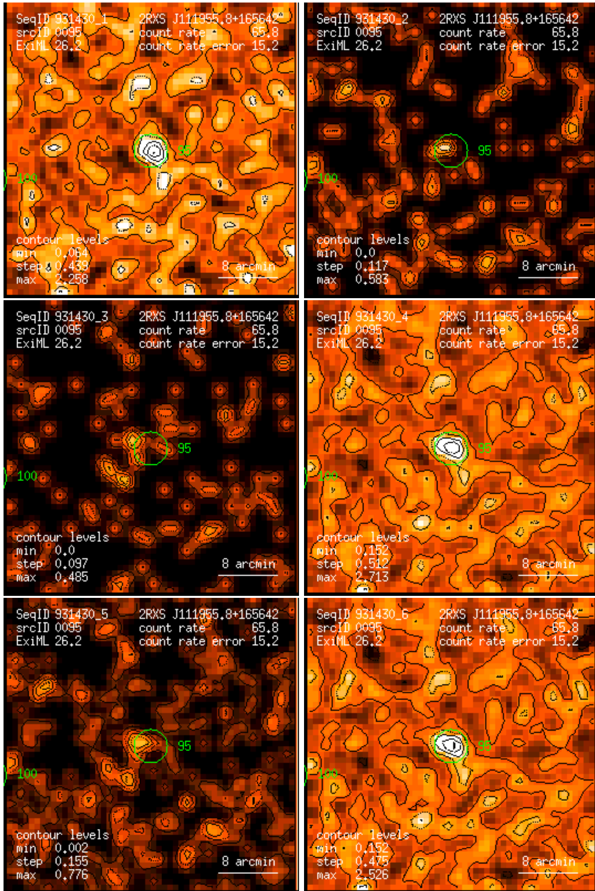
Figure 95: RASS 931430: detection 0095: band rate images, Gaussian filter: (1) PSPC channels 11 – 41, (2) 52 – 90, (3) 91 – 201, (4) 11 – 235, (5) 52 – 201, (6) 11 – 201. Broad band rates in counts/ks. Band rate contour levels in counts/ks/arcmin 2 .
