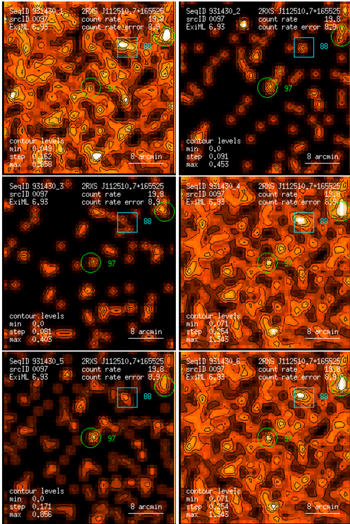
Figure 97: RASS 931430: detection 0097: band rate images, Gaussian filter: (1) PSPC channels 11 – 41, (2) 52 – 90, (3) 91 – 201, (4) 11 – 235, (5) 52 – 201, (6) 11 – 201. Broad band rates in counts/ks. Band rate contour levels in counts/ks/arcmin 2 .
