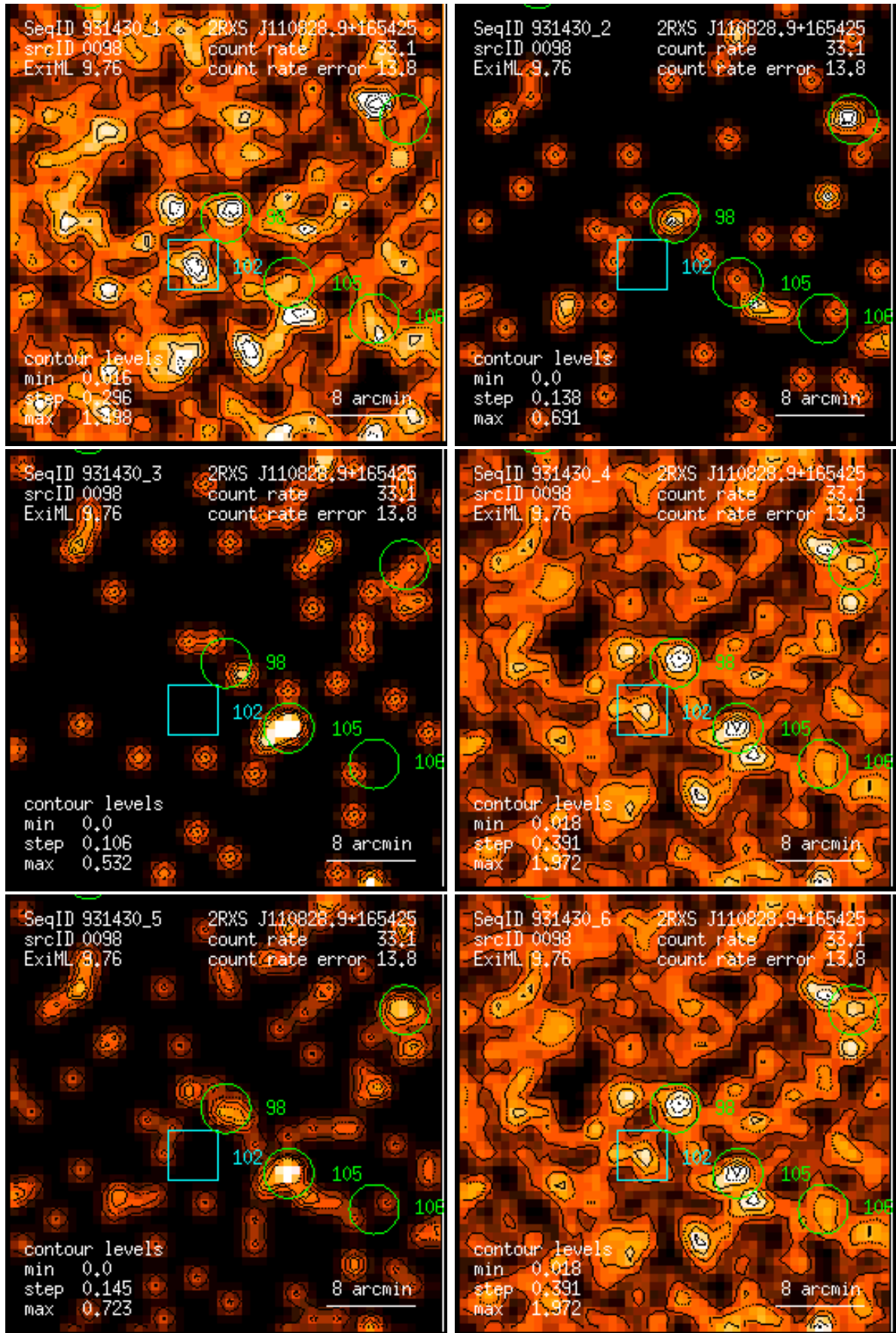
Figure 98: RASS 931430: detection 0098: band rate images, Gaussian filter: (1) PSPC channels 11 – 41, (2) 52 – 90, (3) 91 – 201, (4) 11 – 235, (5) 52 – 201, (6) 11 – 201. Broad band rates in counts/ks. Band rate contour levels in counts/ks/arcmin 2 .
