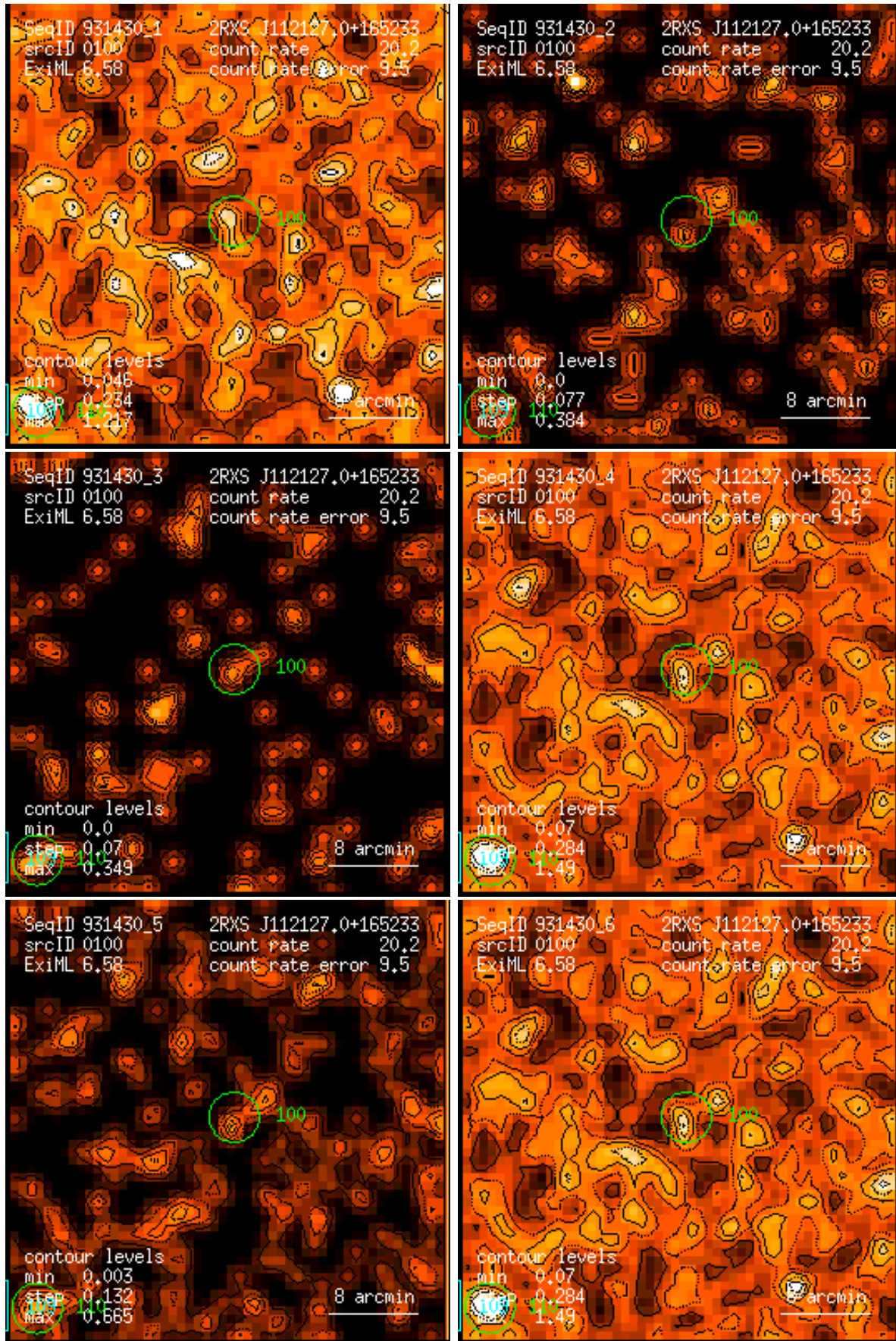
Figure 100: RASS 931430: detection 0100: band rate images, Gaussian filter: (1) PSPC channels 11 – 41, (2) 52 – 90, (3) 91 – 201, (4) 11 – 235, (5) 52 – 201, (6) 11 – 201. Broad band rates in counts/ks. Band rate contour levels in counts/ks/arcmin 2 .
