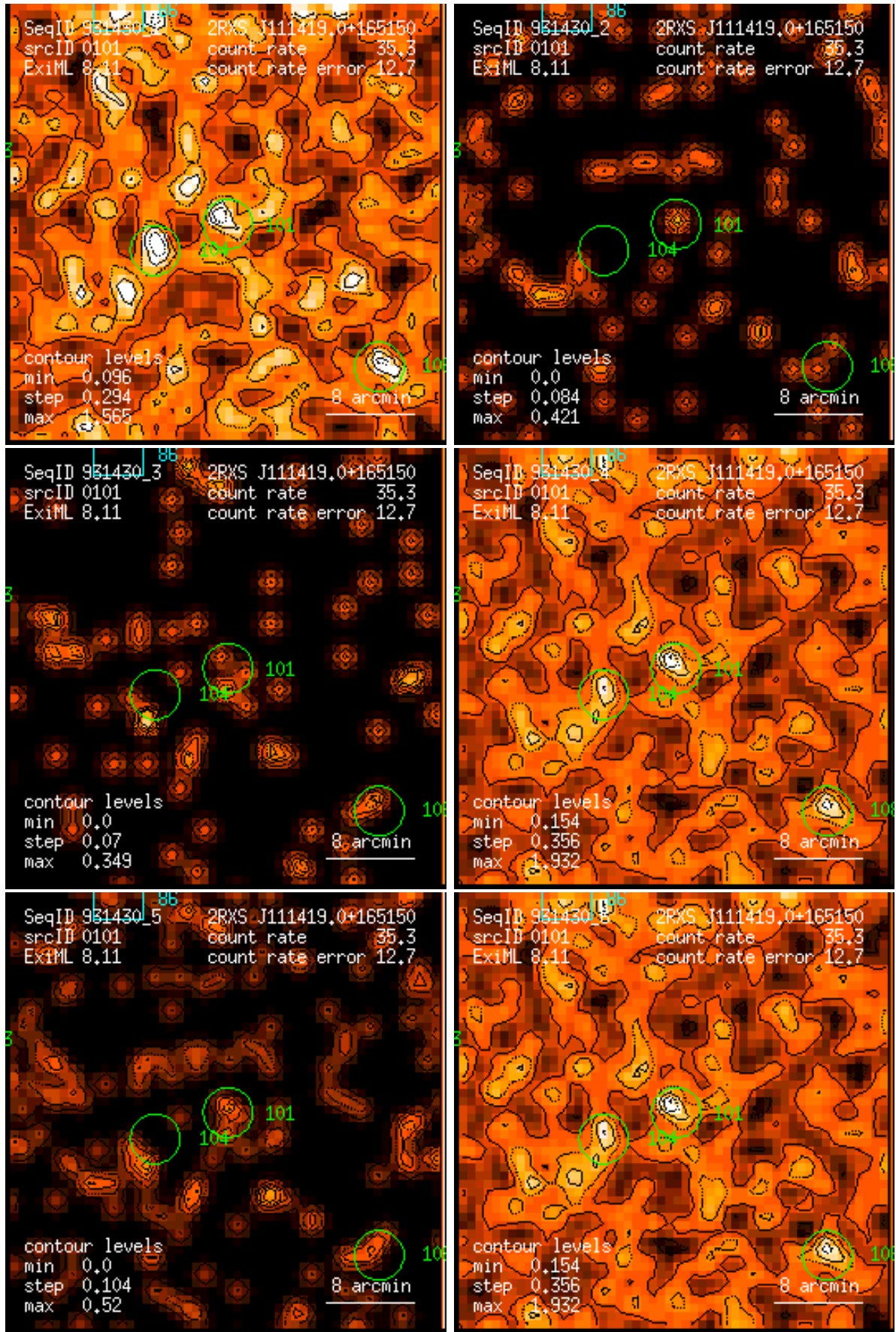
Figure 101: RASS 931430: detection 0101: band rate images, Gaussian filter: (1) PSPC channels 11 – 41, (2) 52 – 90, (3) 91 – 201, (4) 11 – 235, (5) 52 – 201, (6) 11 – 201. Broad band rates in counts/ks. Band rate contour levels in counts/ks/arcmin 2 .
