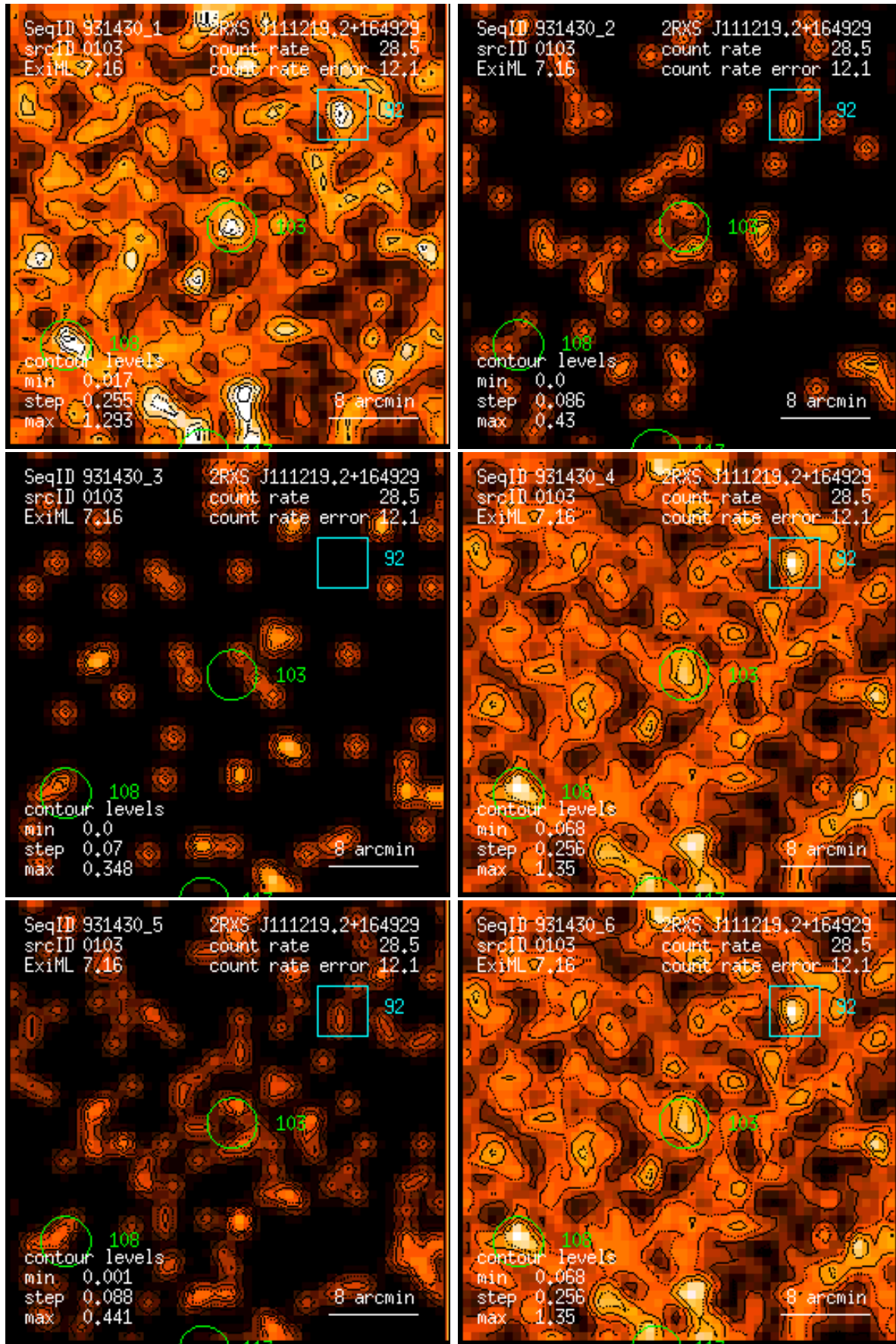
Figure 103: RASS 931430: detection 0103: band rate images, Gaussian filter: (1) PSPC channels 11 – 41, (2) 52 – 90, (3) 91 – 201, (4) 11 – 235, (5) 52 – 201, (6) 11 – 201. Broad band rates in counts/ks. Band rate contour levels in counts/ks/arcmin 2 .
